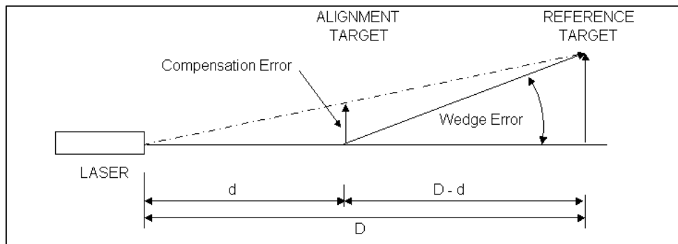
Figure E-2. Two target alignment showing wedge error.
