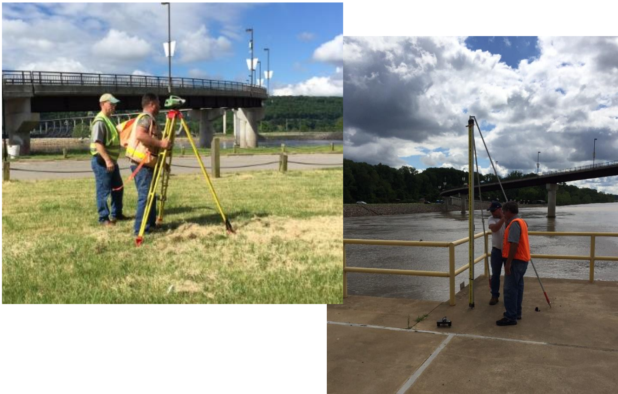
Figure 6-1. Precise leveling runs near/on structure in Little Rock District. (Little Rock District).
