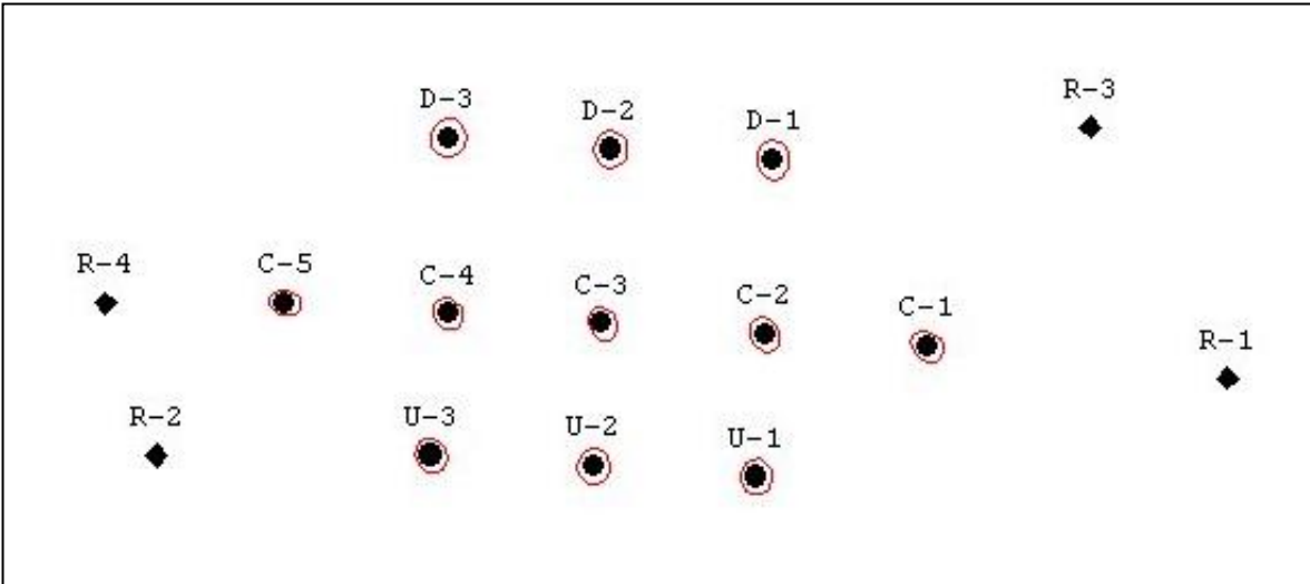
Figure D-2. Adjustment network map (plan view) showing station names, relative locations, and the point confidence ellipse (95%) for horizontal positioning plotted around each point. Network map and confidence ellipses are plotted at different scales. Circles indicate monitoring points and diamonds represent reference stations.
