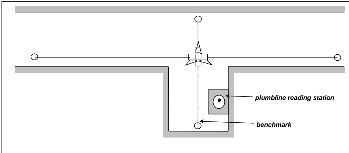
Figure C-14. Tilt measurement with a geodetic level.
