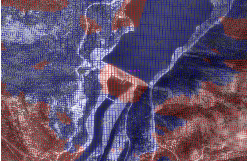
Figure C-2. Intervisibility diagram for reference station placements, blue areas visible, red areas obstructed.
