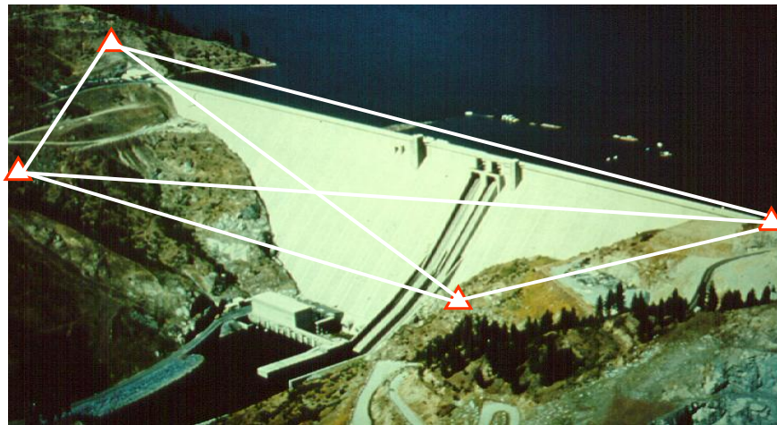
Figure 2-3. Reference network configuration for a concrete dam depicting reference points near abutments and at downstream locations.
