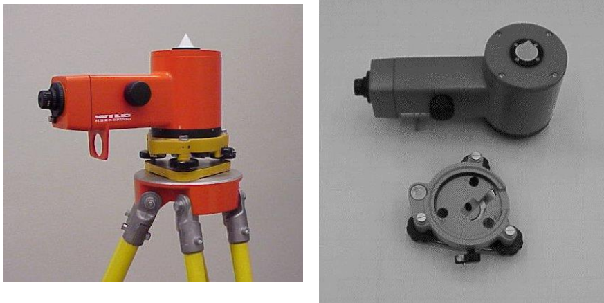
Figure 4-2. Nadir plummet instrument from Leica Co. Nadir plummets operate like an automatic level but establish a vertical LOS. The tribrach is centered over the surveyor's mark using the nadir plummet. Then a theodolite or a GPS antenna is placed in the tribrach by forced centering.
