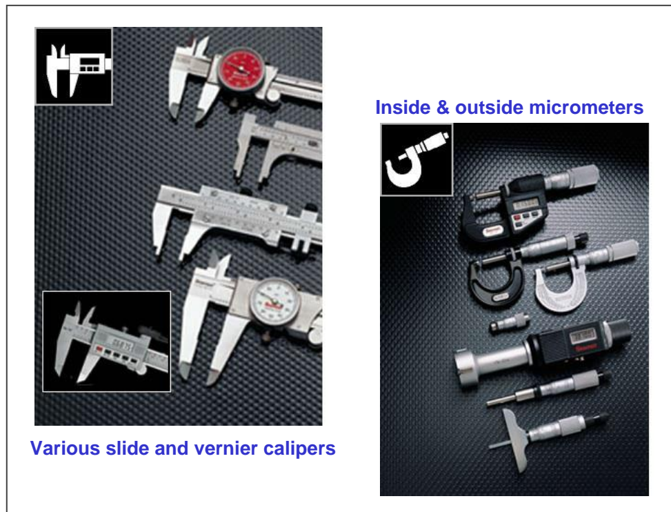
Figure 3-8. Assortment of Starrett micrometers and calipers that can be used for measuring short distances in concrete structures to an accuracy of 0.0005 inch or better.
