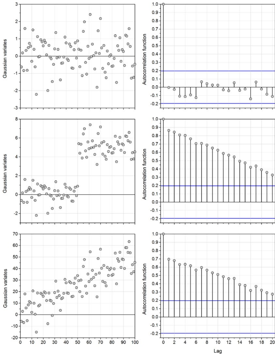
Figure C-1. Examination of the impact of abrupt and linear trends on the autocorrelation function. Top panels: time series of 100 independent standard Gaussian variants (left) and corresponding autocorrelation function. Middle panels: same as the top panel but with the second half of the time series shifted by 5. Bottom panels: same as the top panel but after superimposing a linear trend. The blues lines in the left panels represent the 95% confidence intervals.
