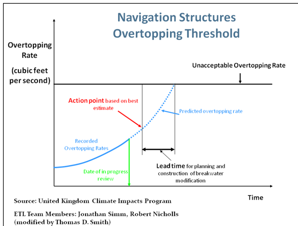
Figure C-3. Tipping point diagram for navigation structure overtopping threshold under a sea level rise scenario
