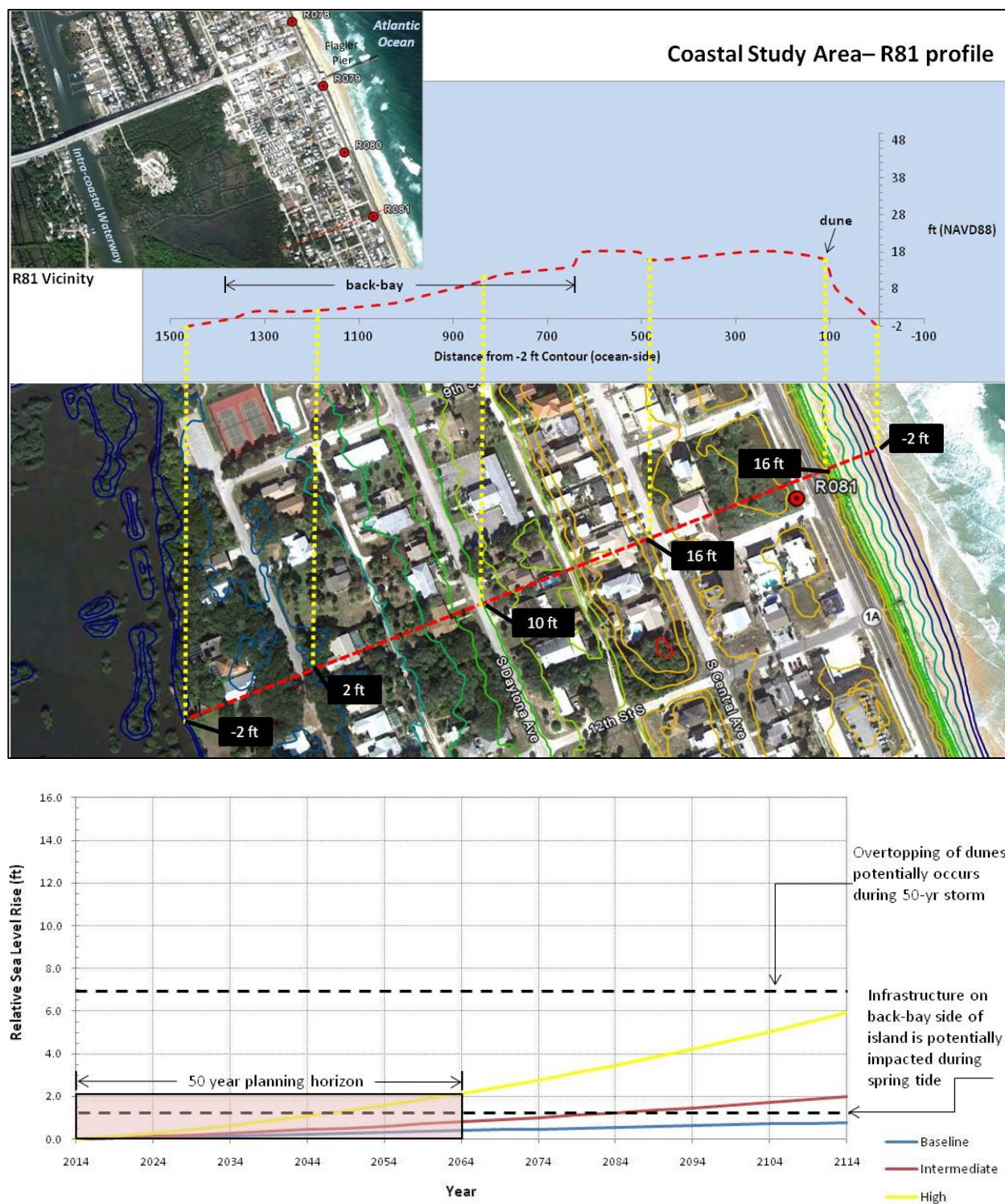
Figure G-3. Project area profile and threshold analysis
