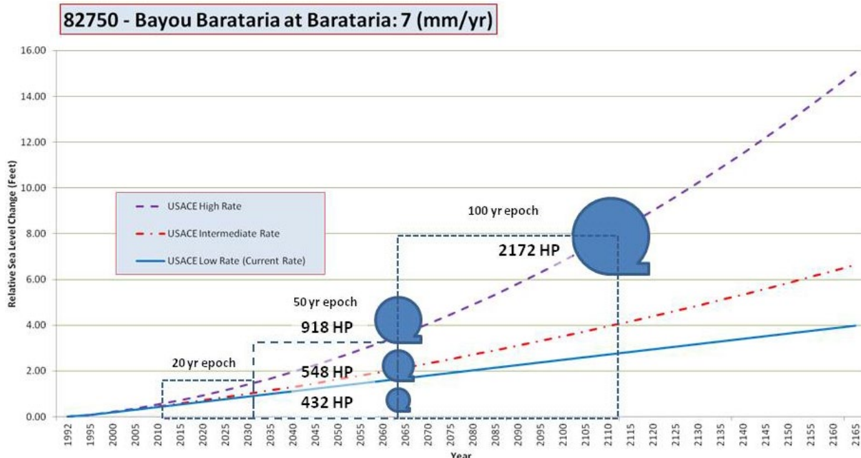
Figure E-13. Algiers SELA pump station capacity required for the three RSLR rates
