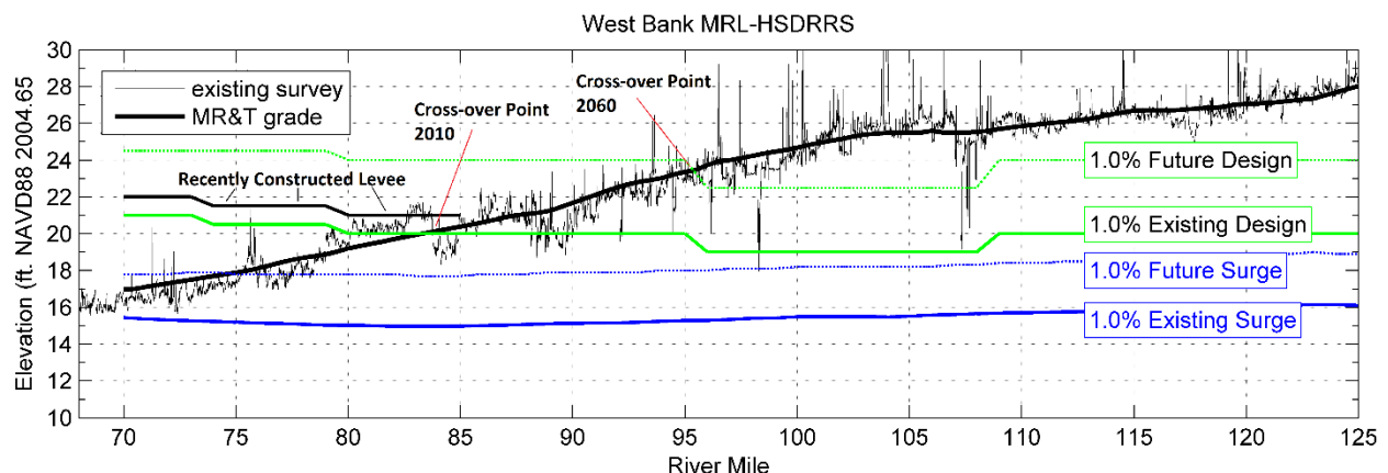
Figure E-4. Example of a moving crossover point for the west (right descending) bank of the Mississippi River near New Orleans. This example assumes a relative sea level rise of 1 ft (0.3m) over 50 years, which, when added into storm surge models, would cause storm surges to increase in height and the coastal storm governing condition to move upstream. A full explanation of the methods of this example can be found in USACE (2011b)
