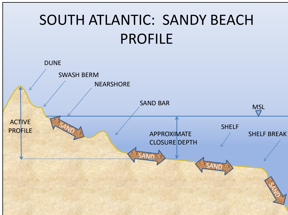
Figure D-5. Typical beach profile for the South Atlantic region (also representative of Gulf of Mexico beaches)
