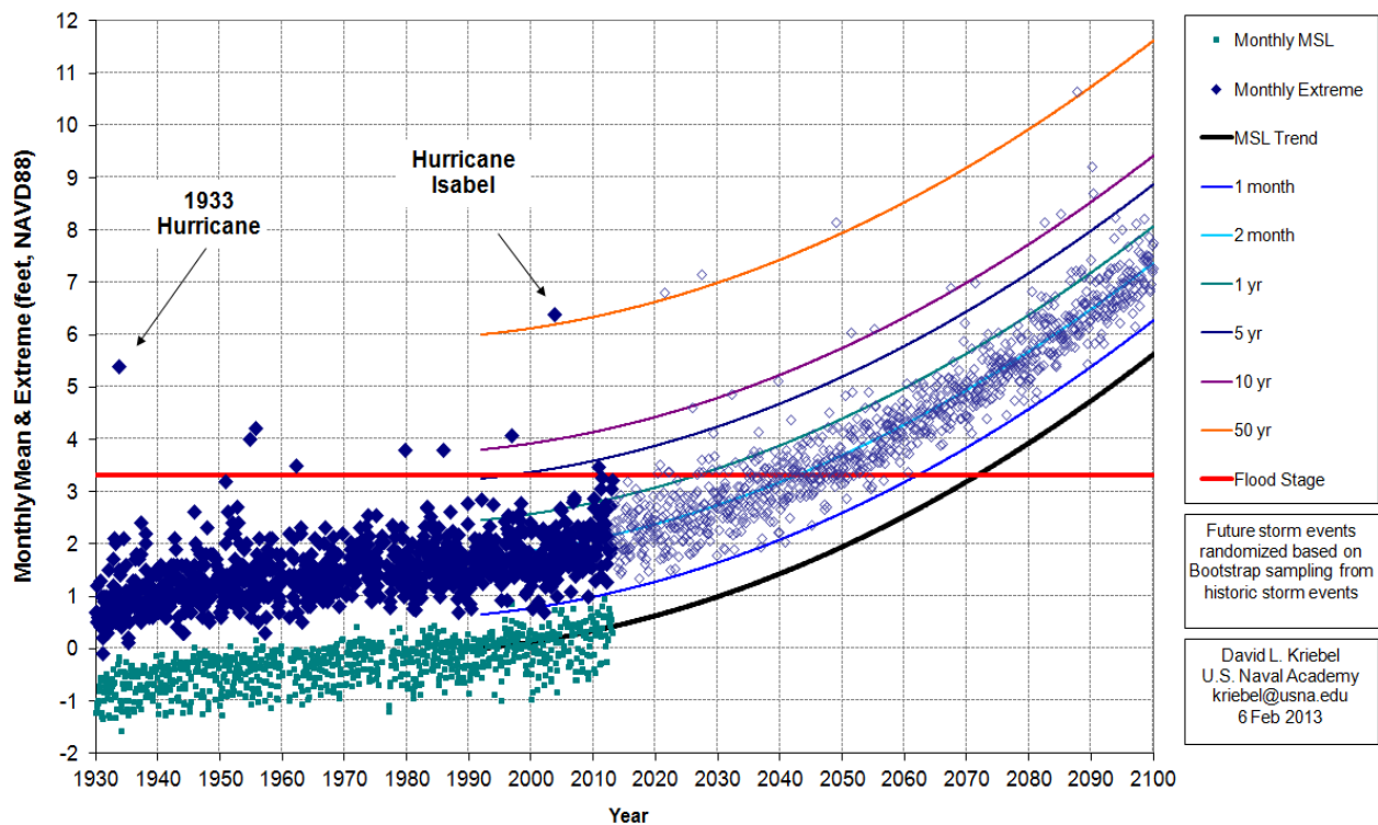
Figure B-21. Future vulnerability to sea level rise (high case) at Annapolis, MD, showing the relationship to local threshold elevations and flood recurrence intervals (From Kriebel 2012.)
