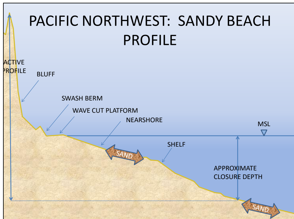
Figure D-3. Typical beach profile for the Pacific Northwest region
