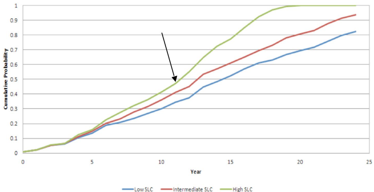
Figure D-1. Cumulative probability of dune rollover at a particular location along a barrier island for low, intermediate, and high SLR rates
