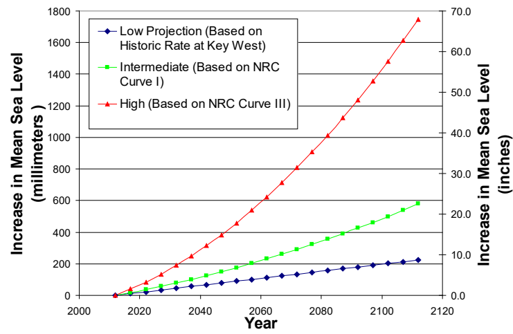
Figure F-3. Projected relative sea level rise at BBCW project features (assuming that construction was completed in 2012)
