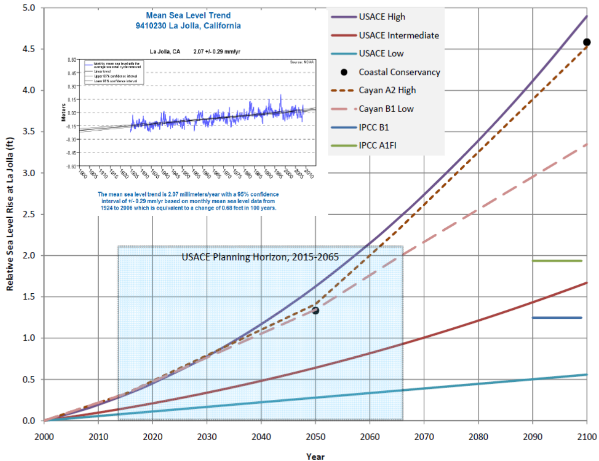
Figure B-15. Comparison of the three sea level rise curves for a USACE project in La Jolla, California
