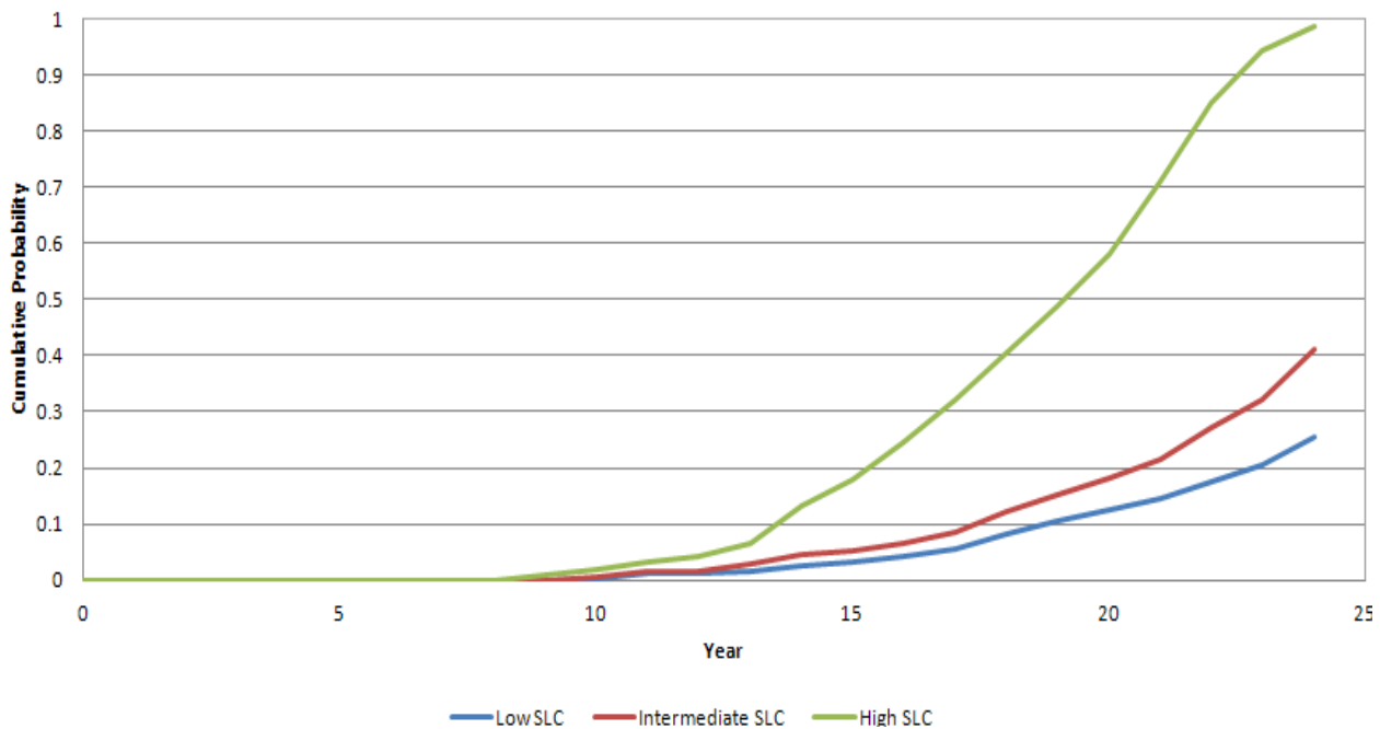
Figure D-2. Cumulative probability of dune crest elevation being lowered
