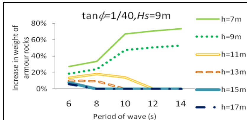
Figure C-8. Increase in the required weight of armor stone for Scenario 4, compared with no SLR (From Esteban et al. 2011.)
