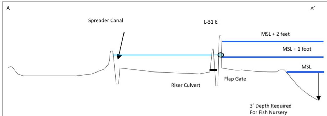
Figure F-4. Homestead Wetlands (Cross section A–A')
