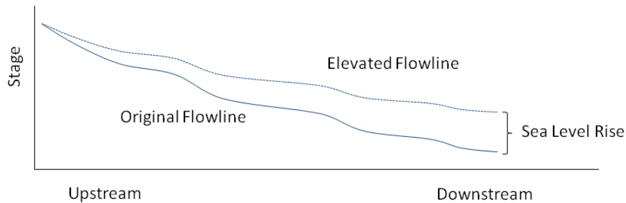
Figure E-2. Backwater effect. As sea levels rise, the downstream boundary stage of a coastal river also rises. This change propagates upstream, causing higher river stages for the same discharge and increasing the frequency of flood stages
