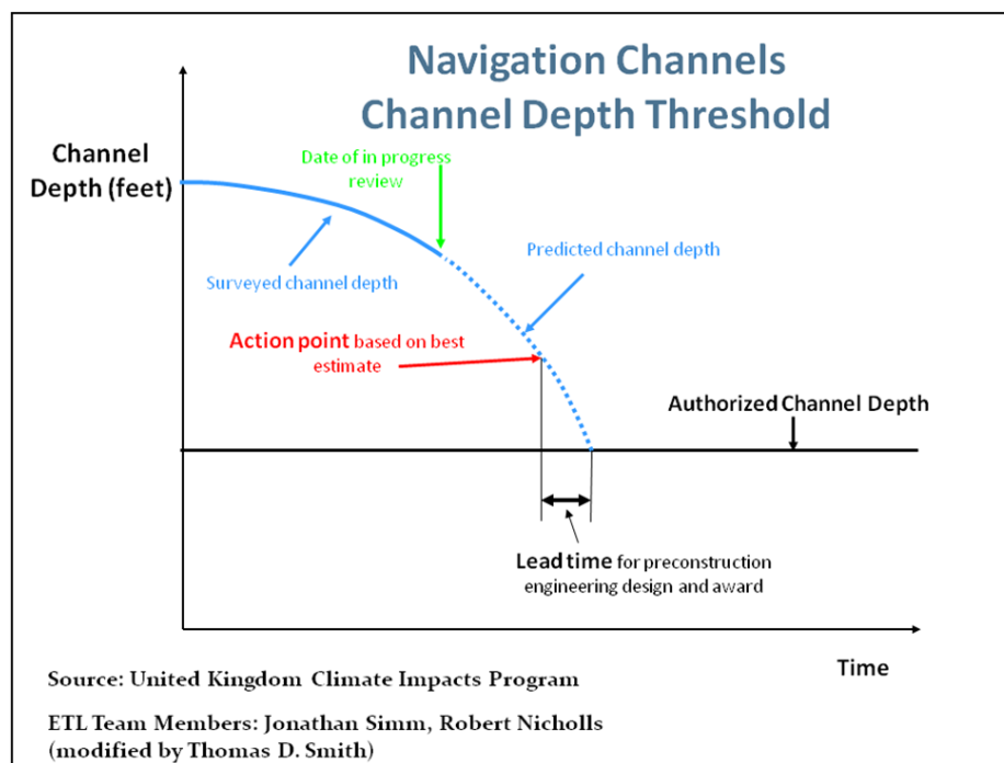
Figure C-5. Tipping point diagram for authorized channel depth under a sea level fall scenario
