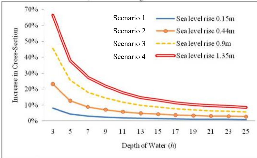
Figure C-6. Increase in breakwater cross section for various sea level rise scenarios. The percent increase in cross section is greater for shallower water depths because the ratio of potential sea level rise to total design water depth is greater along the left side of the figure (From Esteban et al. 2011.)
