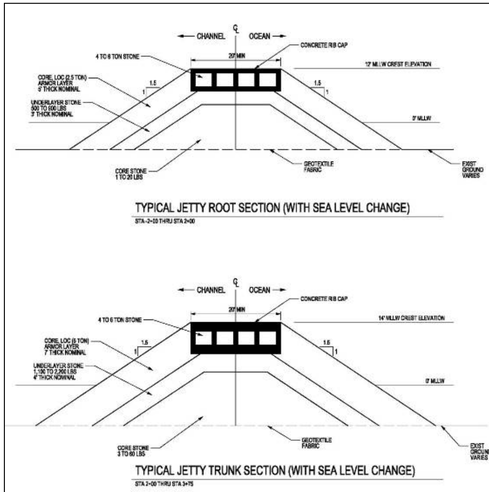
Figure C-17. Typical jetty root and trunk section design based on the USACE high curve for sea level rise at Barbers Point Harbor (From USACE 2012.)
