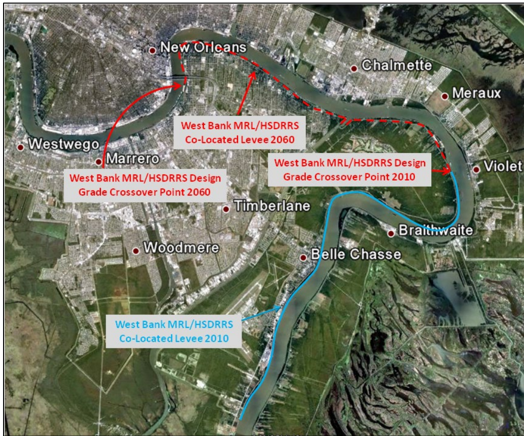
Figure E-5. Location of present and future crossover points between the riverine-governed and coastal-surge-governed flood risk reduction infrastructure near New Orleans (assuming 1ft (0.3m) of relative sea level rise). This figure is based on the results shown in Figure E-4
