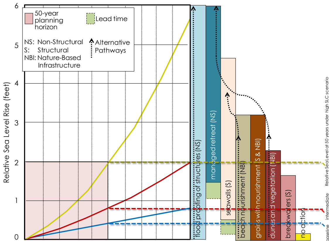
Figure 16. Example alternative pathways for a coastal storm damage reduction project
