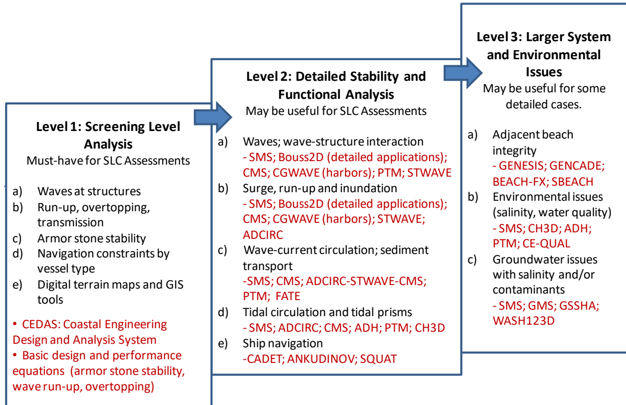
Figure C-12. Graduated levels of USACE analysis tools and modeling techniques
