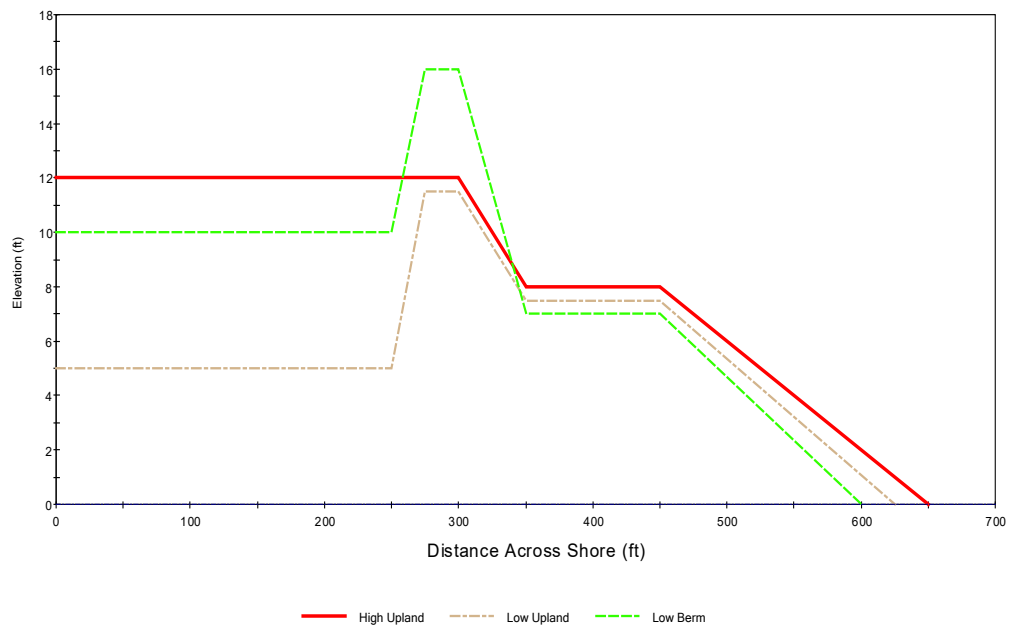
Figure D-9. General beach morphology types: high upland, low upland, and low berm
