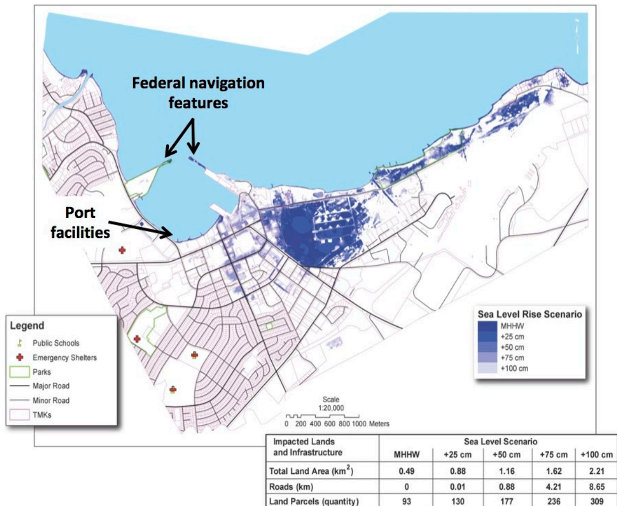
Figure C-1. Example layout of a navigation project with impacted features and areas noted (From Cooper et al. 2012.)
