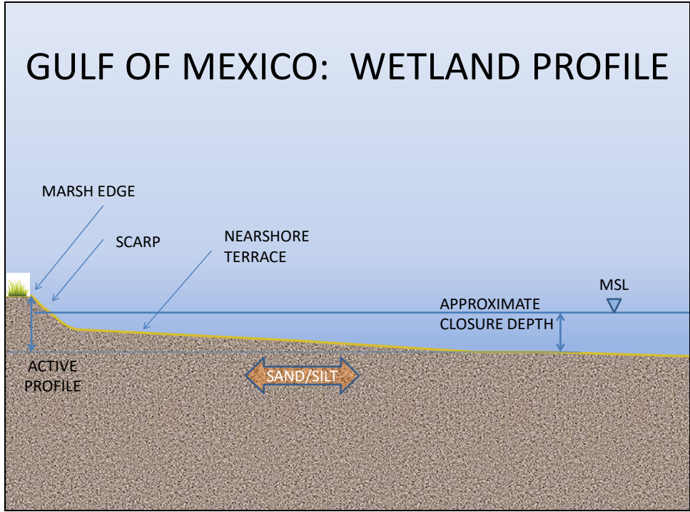
Figure D-6. Typical beach profile for the Gulf of Mexico region
