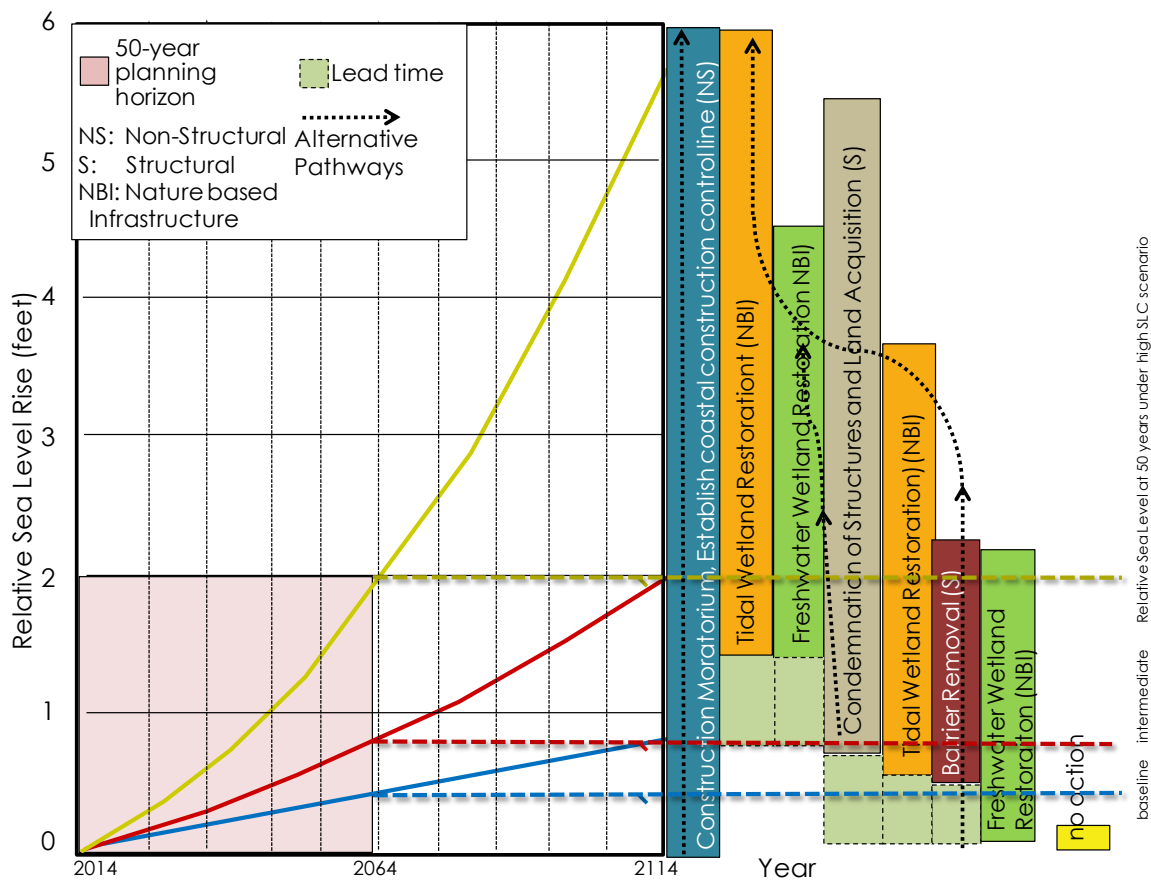
Figure F-1. Example of an adaptive plan for a wetland restoration project subject to SLC
