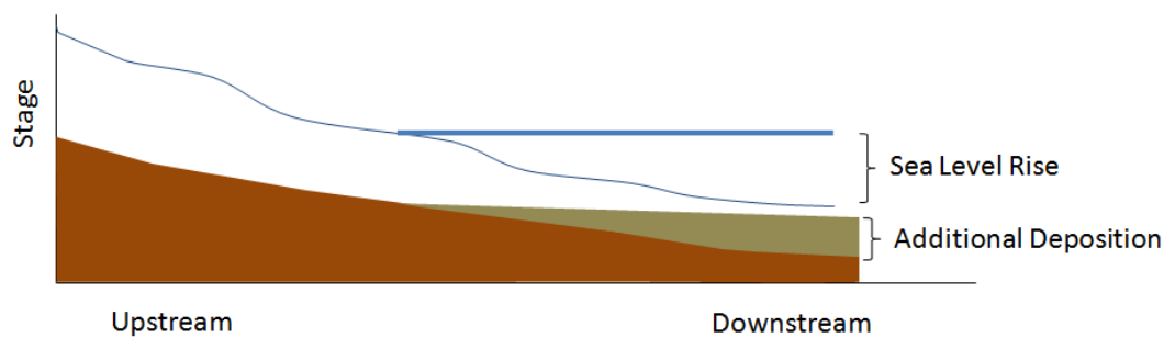
Figure E-3. River channel geometry change. SLC can alter the hydraulic slope and bottom shear stress, altering sediment transport and causing river channels to gain or lose cross section. The resulting change in the stage–discharge relationship alters the frequency of flood stages
