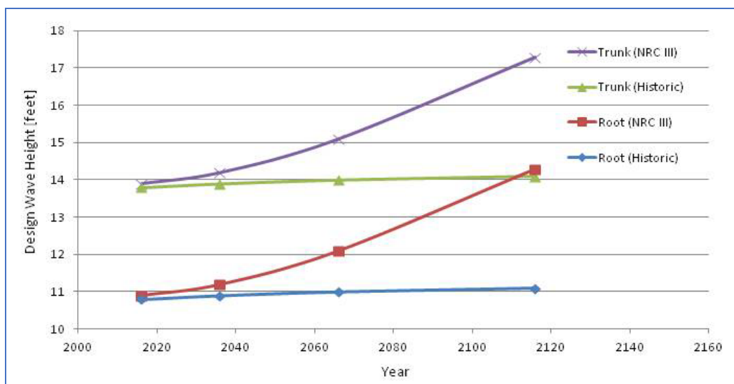
Figure C-15. Depth-limited breaking wave heights (with SLC)
