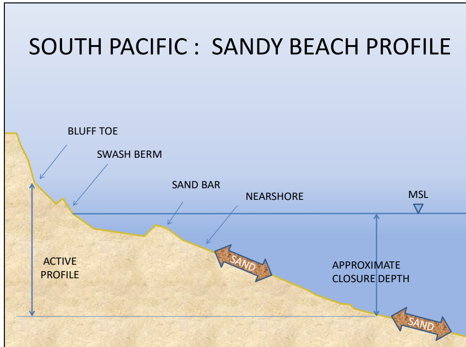
Figure D-4. Typical beach profile for the South Pacific region
