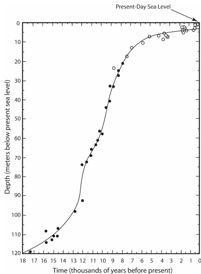
Figure B-2. Rise in global mean sea level over the last 18,000 years (From Williams et al. 2009.)
