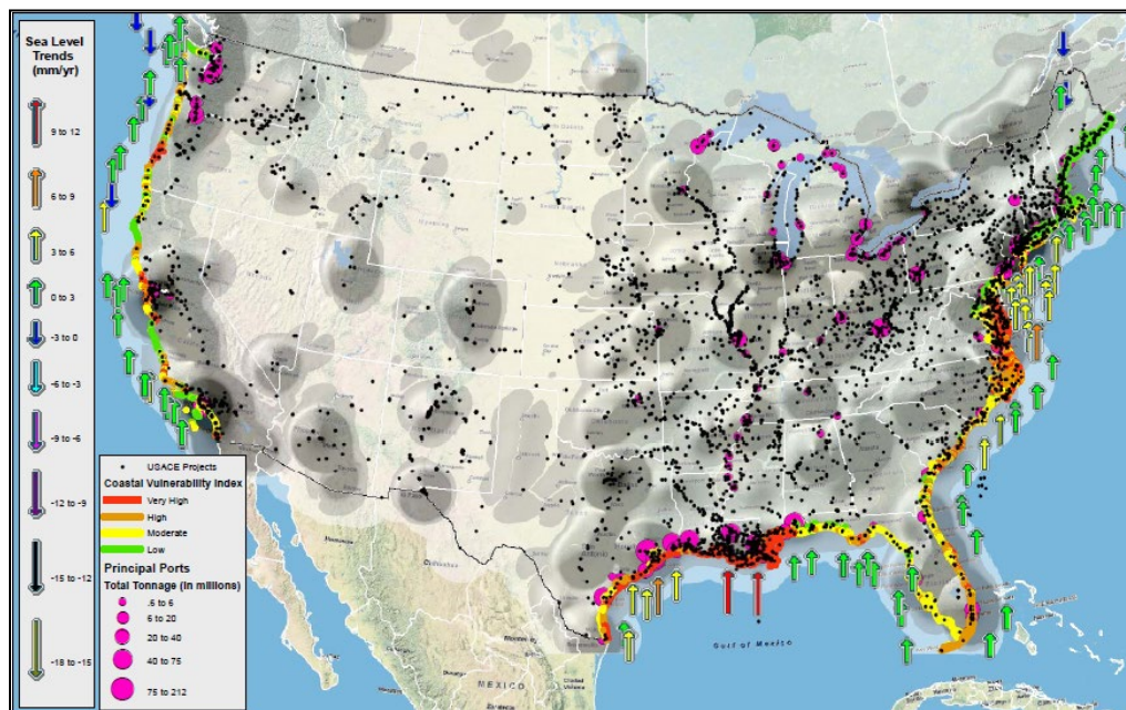
Figure 12. National map illustrating all USACE project locations, NOAA sea level trends, and USGS Coastal Vulnerability Index values. The gray relief shown in the figure (light to dark) indicates population density
