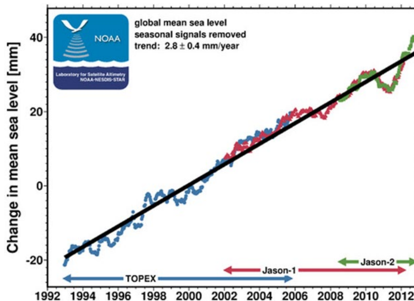
Figure B-4. Estimated rate of global sea level rise since 1993 using satellite altimeter data (From NOAA 2012.)
