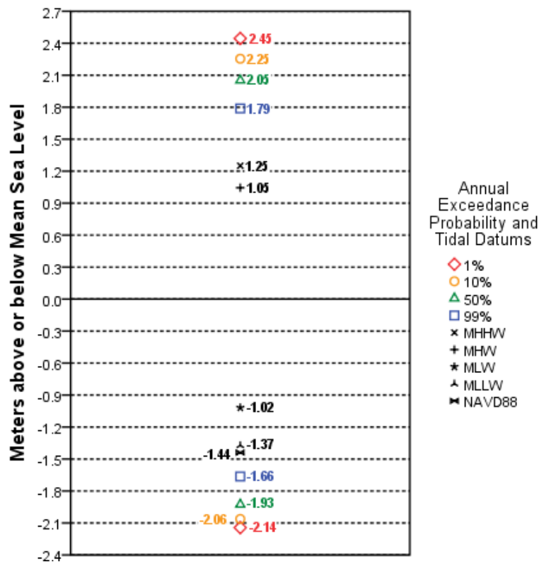
Figure B-17. Stick diagram of exceedance probability levels for Astoria, OR ( http://tidesandcurrents.noaa.gov/est/stickdiagram.shtml?stnid=9439040 .)
