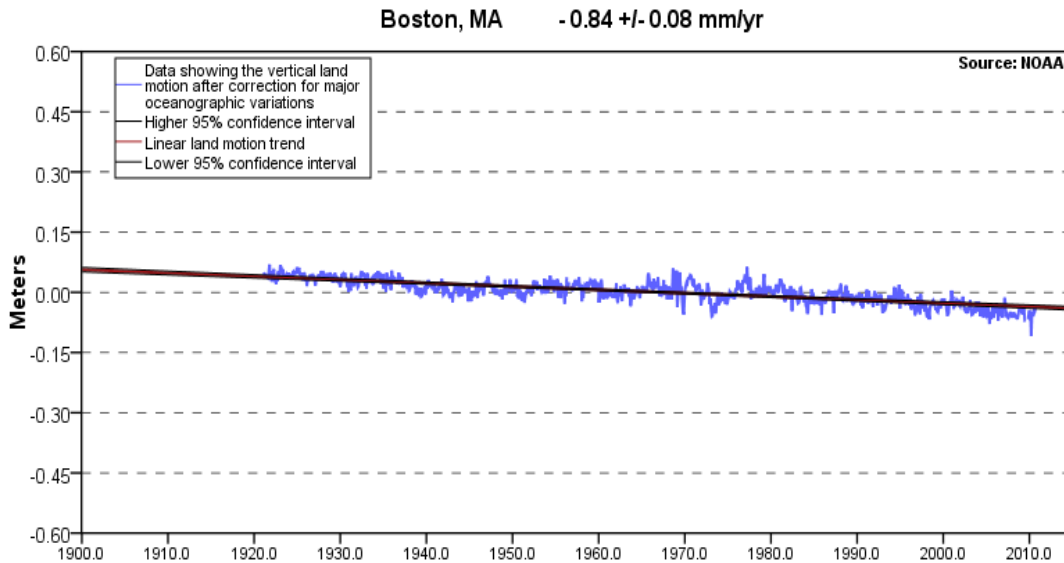
Figure B-14. Estimated vertical land motion at Boston, MA
