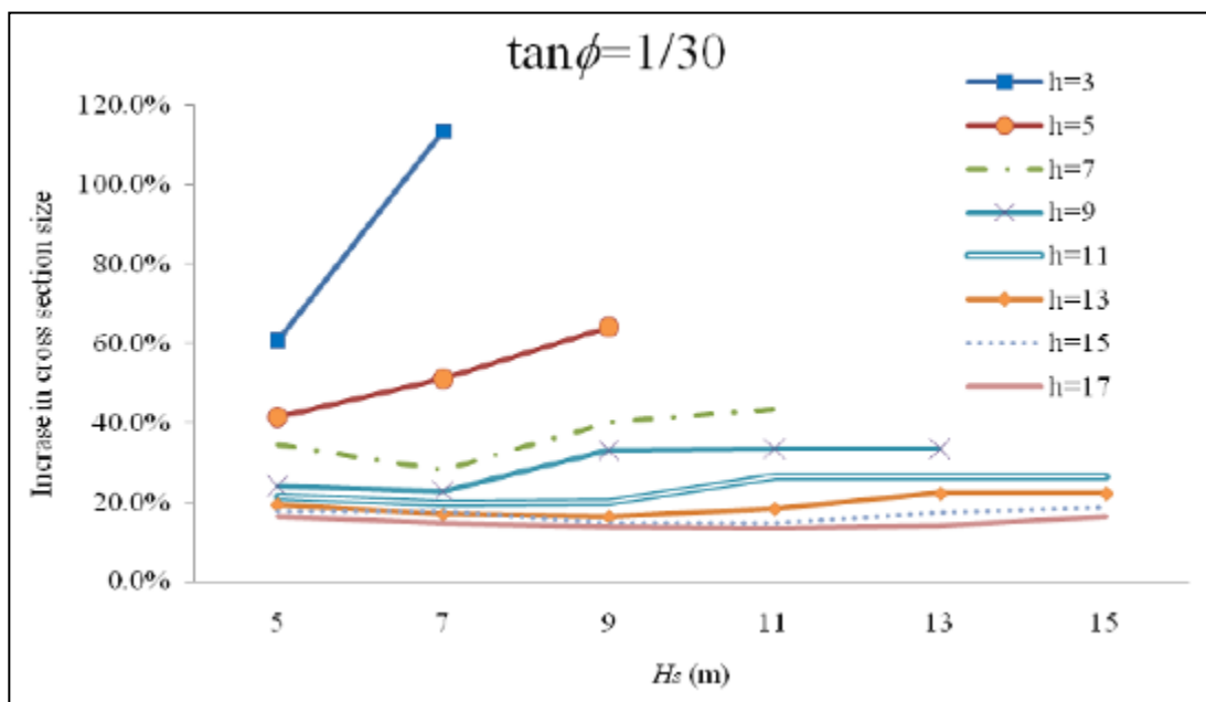
Figure C-10. Increase in cross section of structure for Scenario 4 for a variety of H_s values (From Esteban et al. 2011.)
