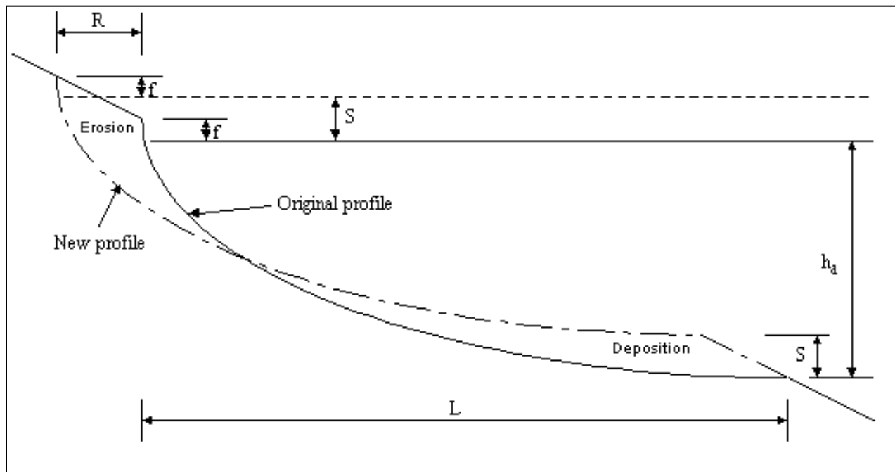
Figure D-8. Diagram of the Bruun Rule method for estimating the beach profile response to SLR
