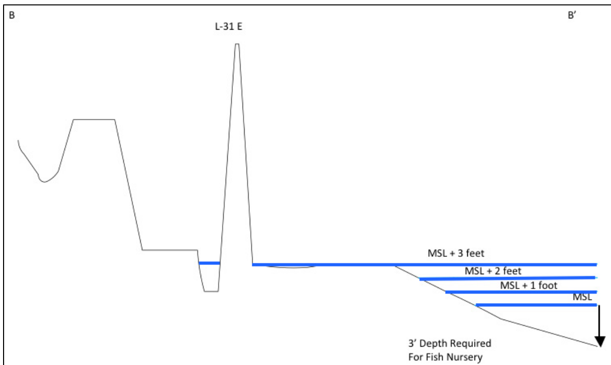
Figure F-5. L-31E Cutler Wetlands (Cross section B–B')
