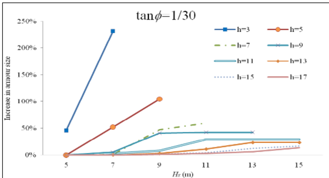
Figure C-9. Increase in armor stone size for Scenario 4 for a variety of H_s values (From Esteban et al. 2011.)
