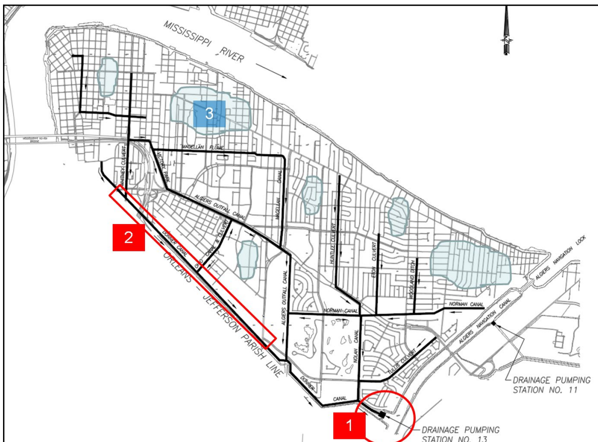
Figure E-10. Algiers catchment showing primary design elements and topographic aspects of the catchment sensitive to RSLR: (1) pump station capacity/efficiency, (2) drainage channel conveyance, and (3) higher water tables due to subsidence
