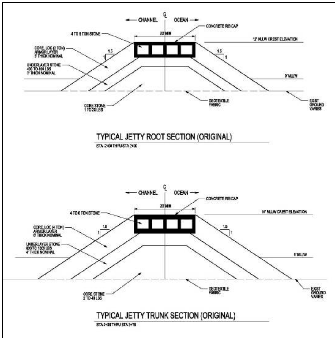
Figure C-14. Typical sections for the original jetty design (without consideration of SLC) (From USACE 2012)
