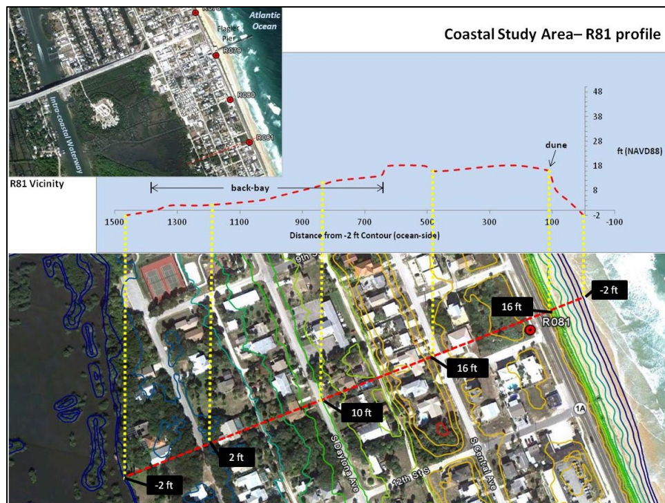
Figure G-1. Project area profile
