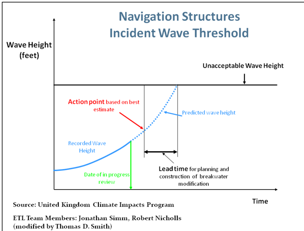
Figure C-2. Activities required under an adaptive strategy to prevent reaching a tipping point at which wave height becomes unacceptable
