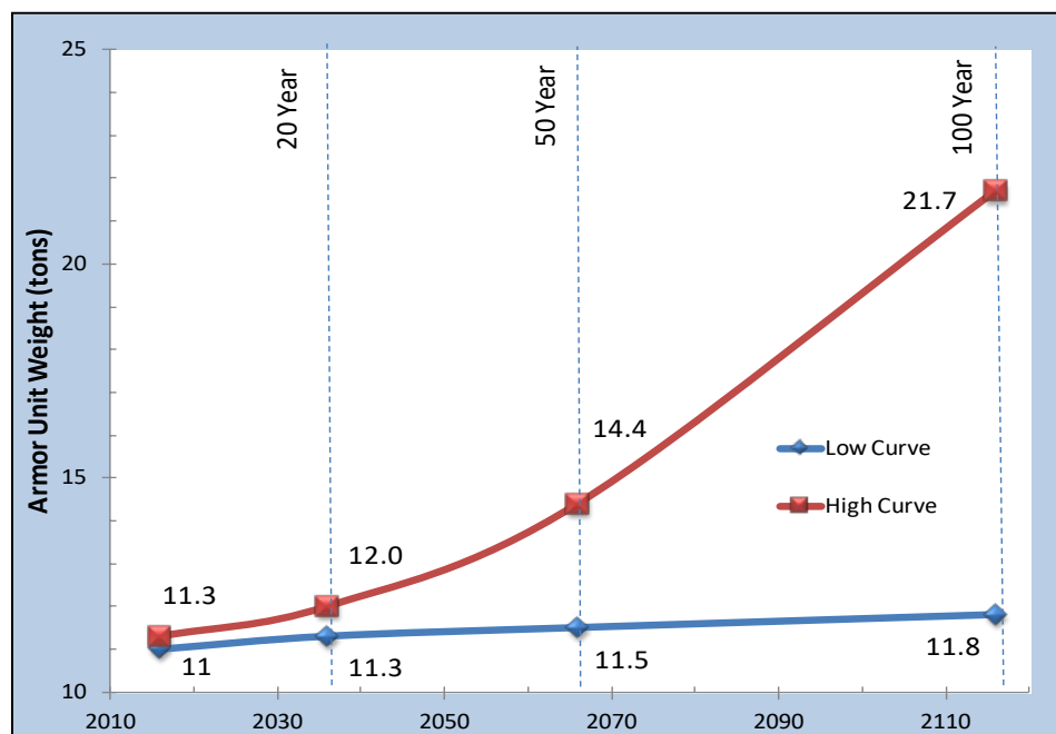
Figure 15. Sensitivity to SLC of frontside design armor for a rubble-mound structure (EM 1110-2-1100)
