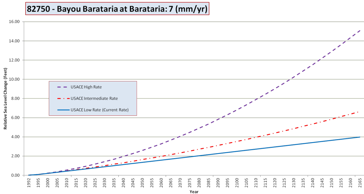
Figure E-8. Relative sea level rise curves for the nearest long-term tide gauge
