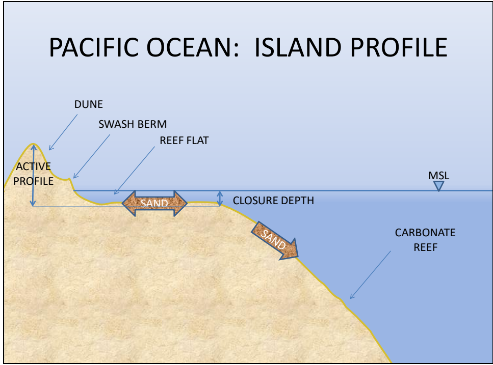
Figure D-7. Typical beach profile for the Pacific Islands region
