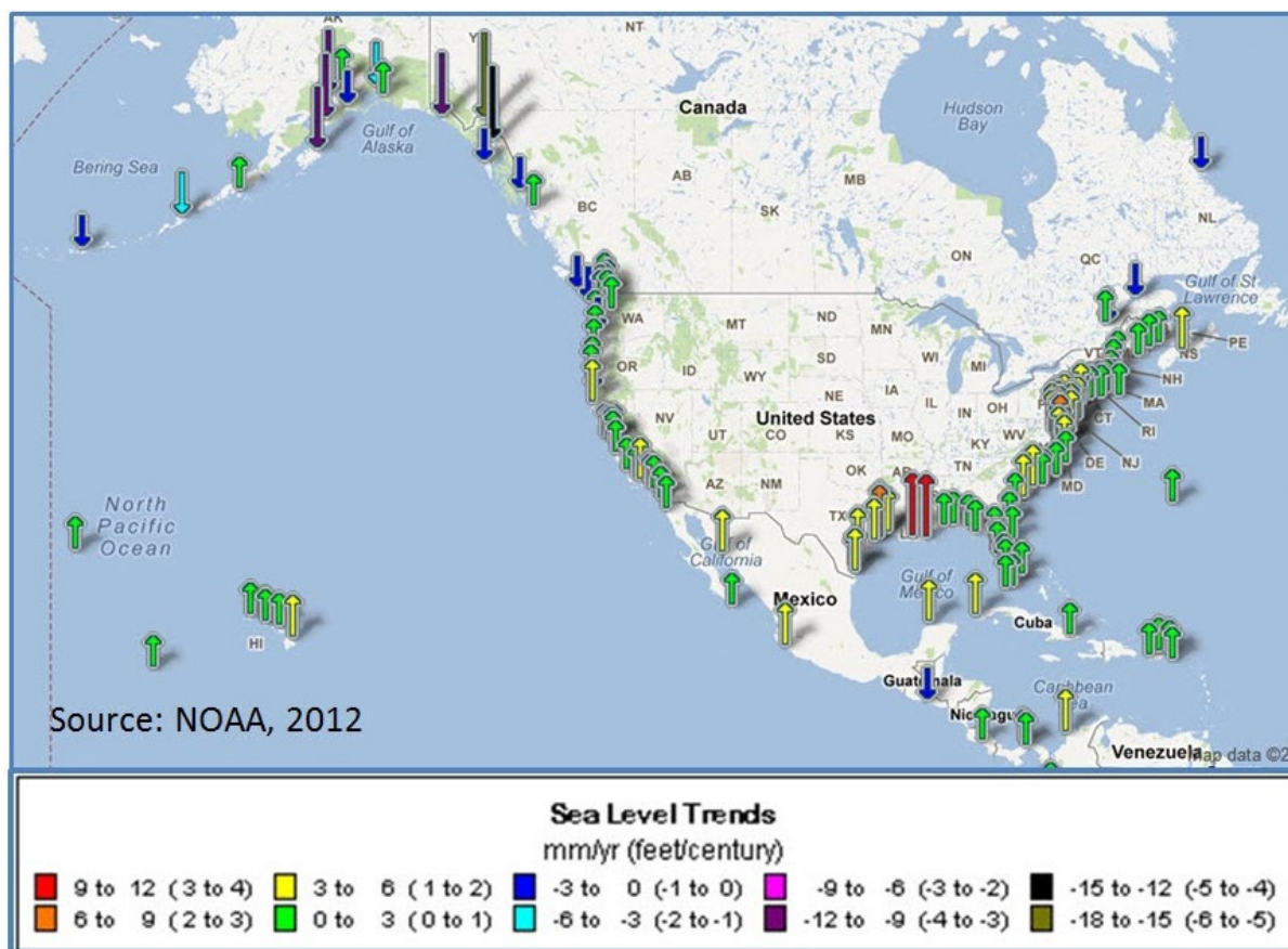
Figure B-7. Mean sea level trends for U.S. tide stations (NOAA 2011). See http://tidesandcurrents.noaa.gov/sltrends/slrmap.html for updated information
