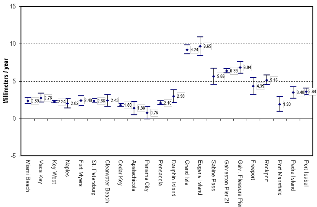
Figure B-10. Magnitude and confidence limits of trends for Florida Keys and Gulf of Mexico coast NOS tide gauges (From Zervas 2009.)
