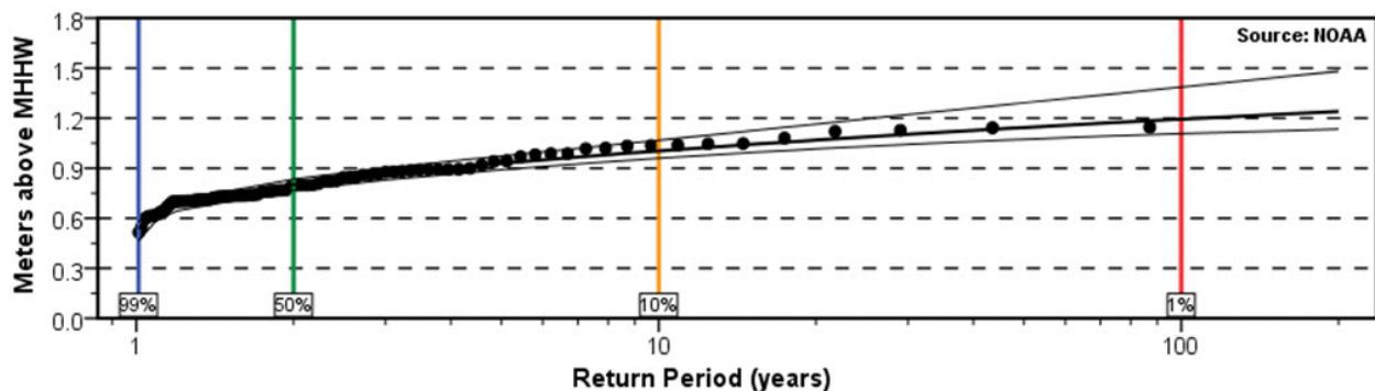
Figure B-18. Annual exceedance probability curve for Astoria, OR ( http://tidesandcurrents.noaa.gov/est/curves.shtml?stnid=9439040 .)
