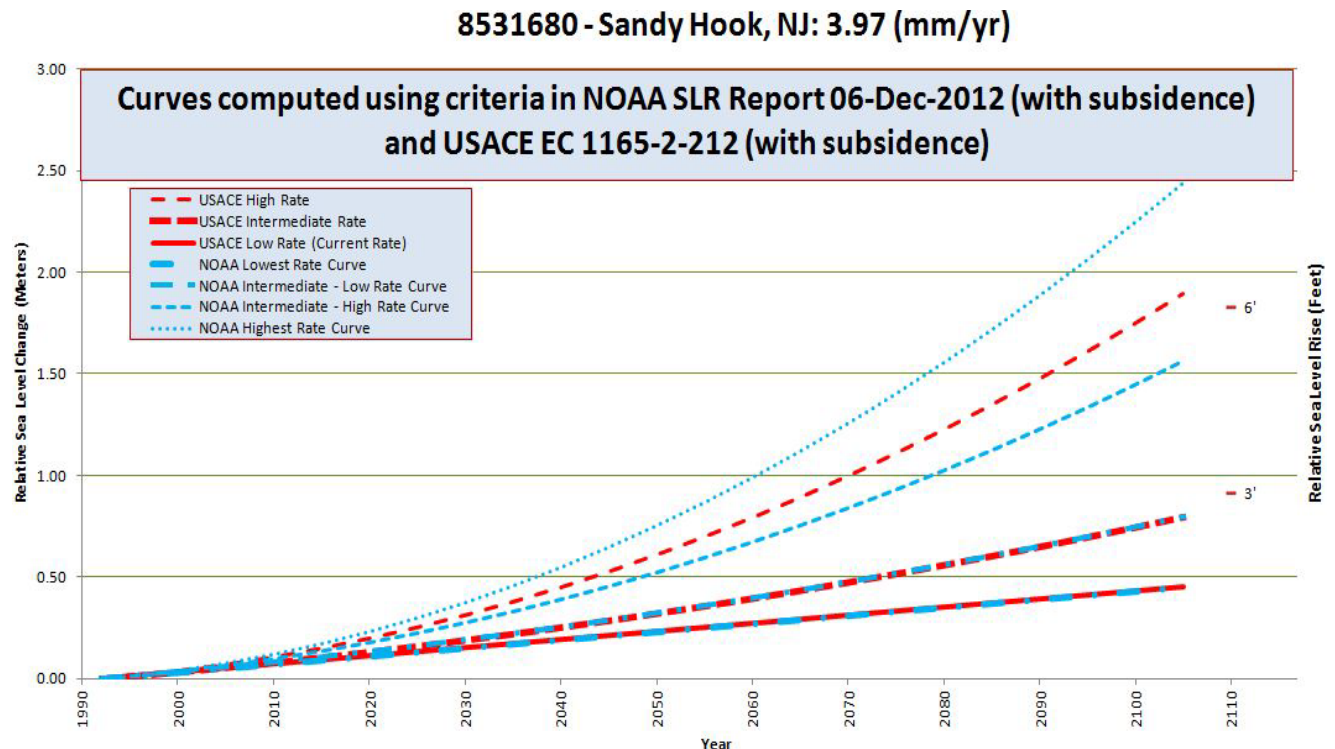
Figure B-16. Graphical comparison of the NRC and National Climate Assessment (NCA) sea level rise scenario curves (NRC I and NCA Intermediate Low curves are the same) using the USACE sea level rise calculator ( http://corpsmapu.usace.army.mil/rccinfo/slc/slcc_calc.html )
