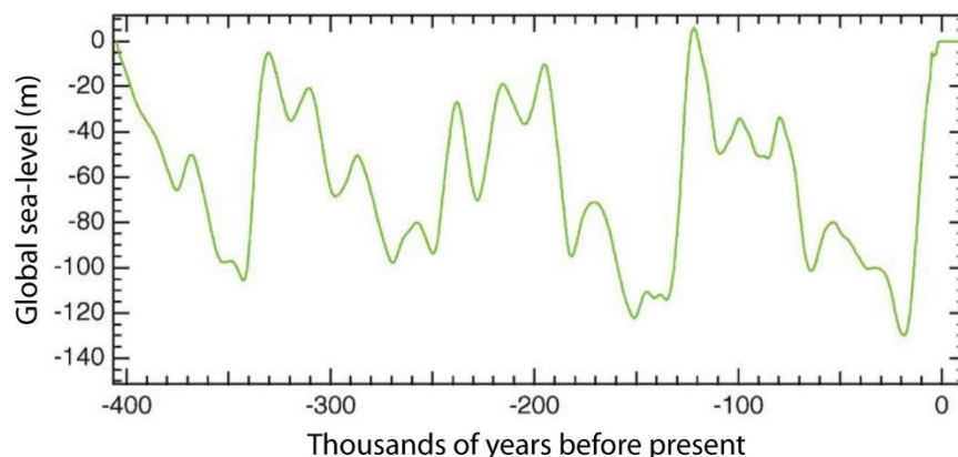
Figure B-1. Global sea level change from 400,000 years ago to the present. (From Williams et al. 2009.)
