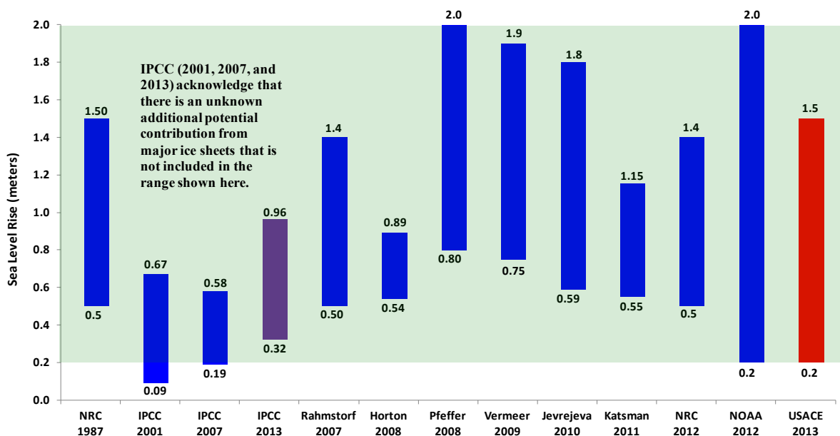
Figure 2. Comparison of maximum and minimum estimates of global sea level rise by 2100
