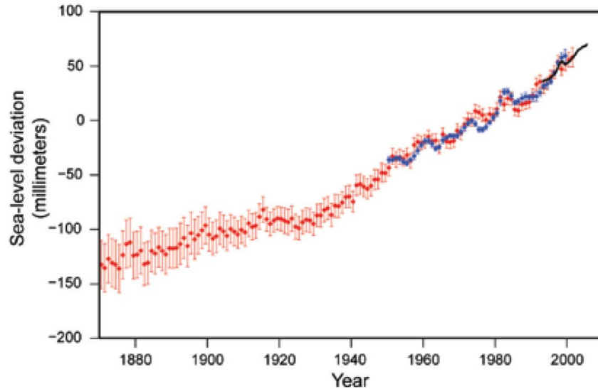
Figure B-3. Global mean sea level change since 1860 [From Williams et al. 2009 (modified from IPCC 2007)]
