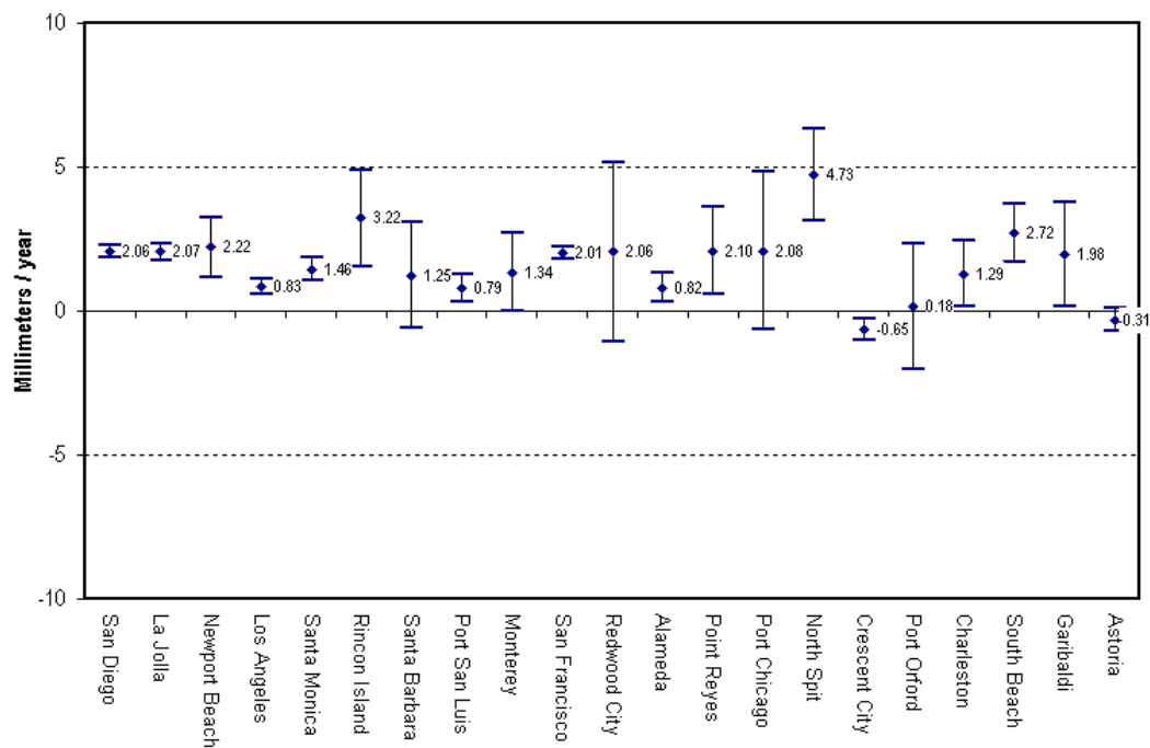
Figure B-11. Magnitude and confidence limits of trends for southern Pacific coast NOS tide gauges (From Zervas 2009.)
