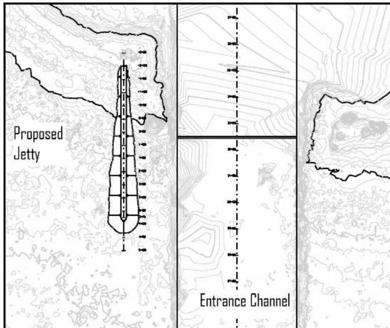
Figure C-13. Proposed jetty alignment relative to the Barber Point Harbor entrance channel (From USACE 2012)
