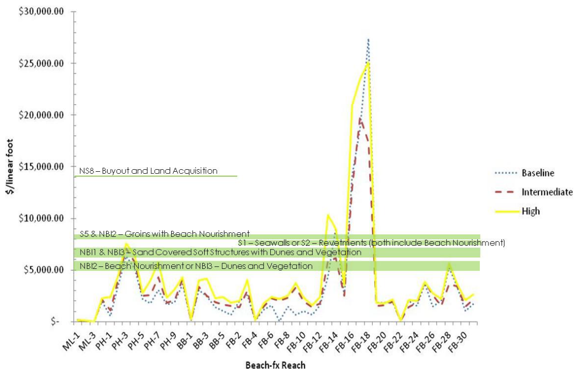
Figure G-7. Management measure costs plotted against future without-project damages along the study area shoreline
