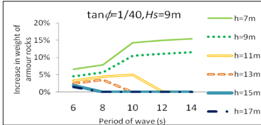
Figure C-7. Increase in the required weight of armor stone for Scenario 2, compared with no SLR (From Esteban et al. 2011.)
