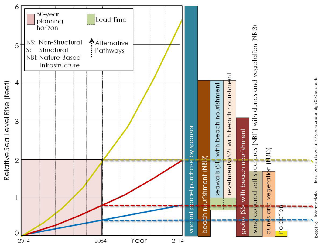
Figure G-8. Alternative adaptability to SLC scenarios
