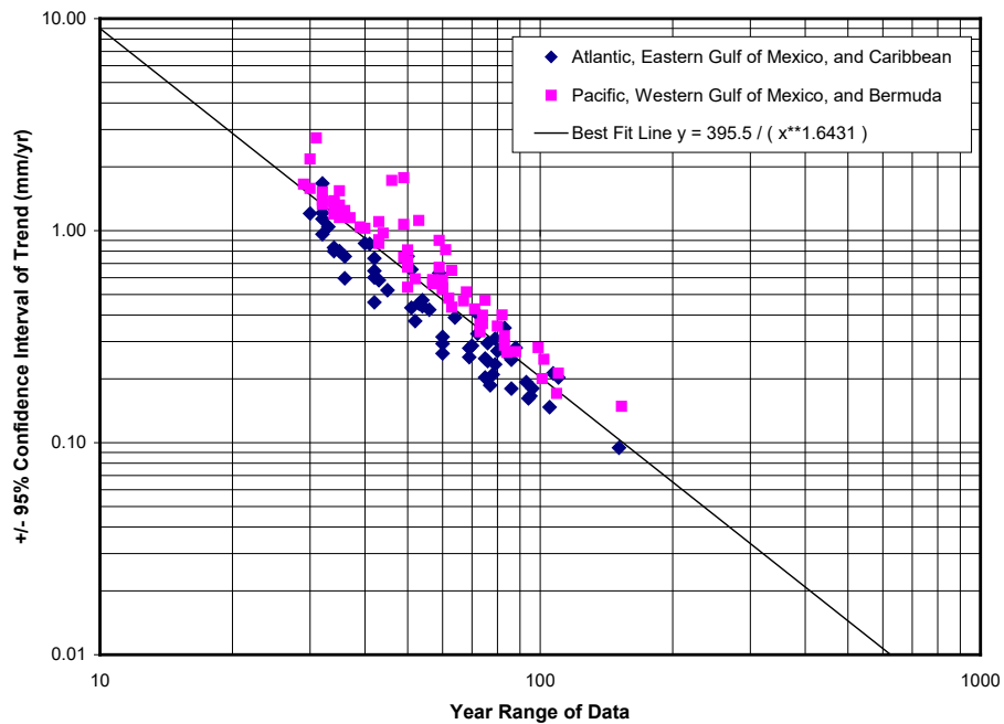
Figure B-9. \pm 95% confidence interval of linear MSL trends (mm/yr) vs. year range of data. The least-squares fitted line is also shown (From Zervas 2009.)
