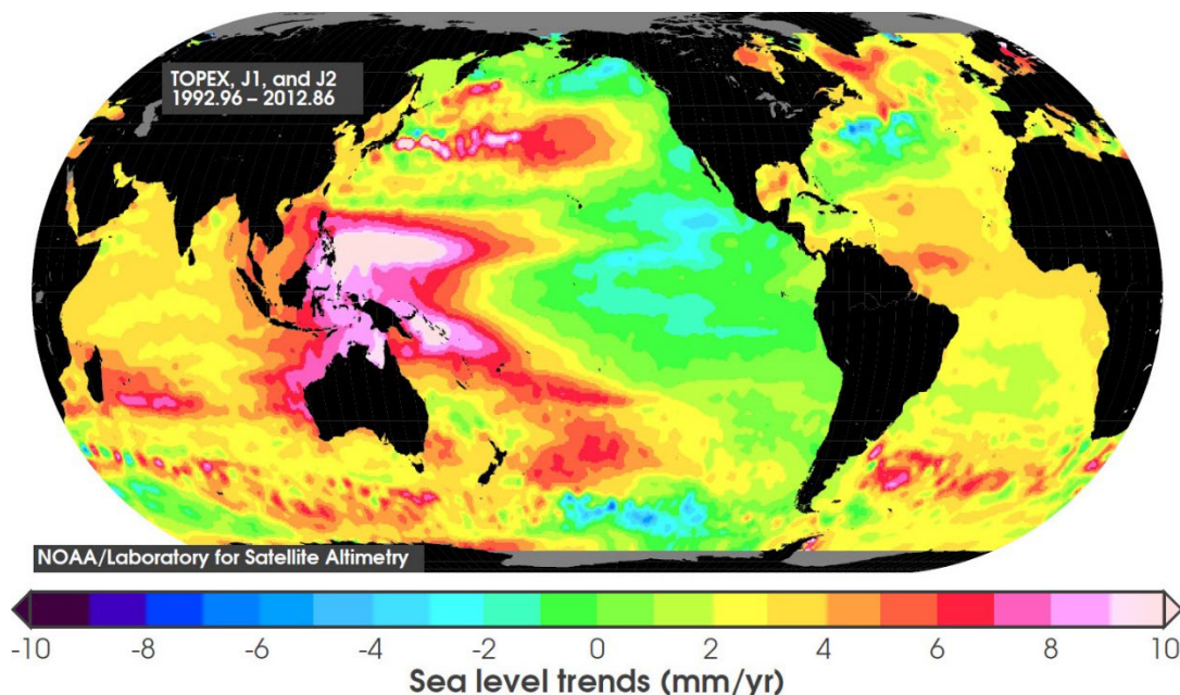
Figure B-5. Regional rates of sea level change between 1993 and present from overlapping satellite altimeter missions (From NOAA 2010b.)
