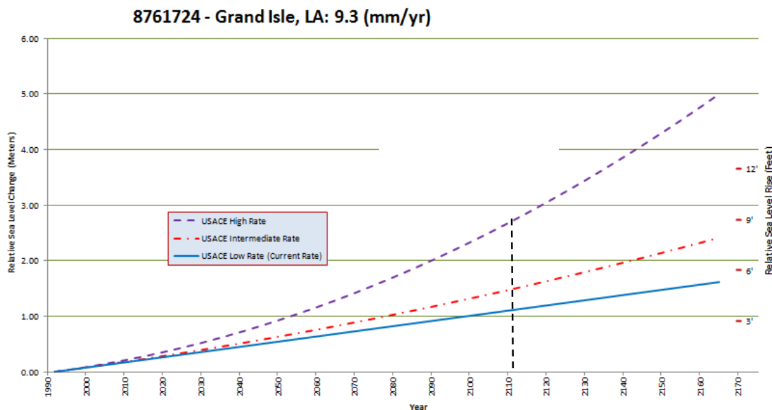
Figure 3. USACE SLC curves for Grand Isle, Louisiana. These curves include eustatic sea level rise values and subsidence rates
