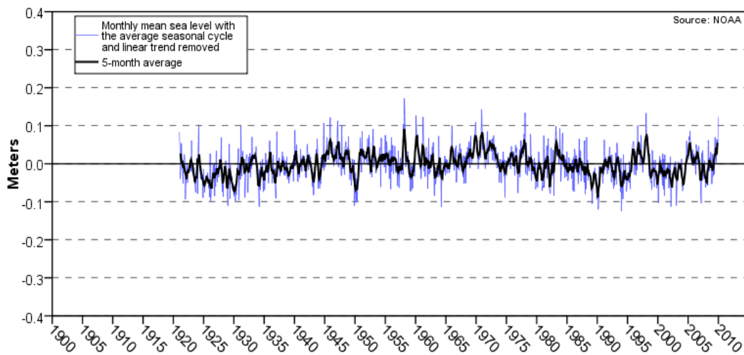
Figure B-13. Regional oceanographic residual using an average of the data from Eastport, ME, to Boston, MA
