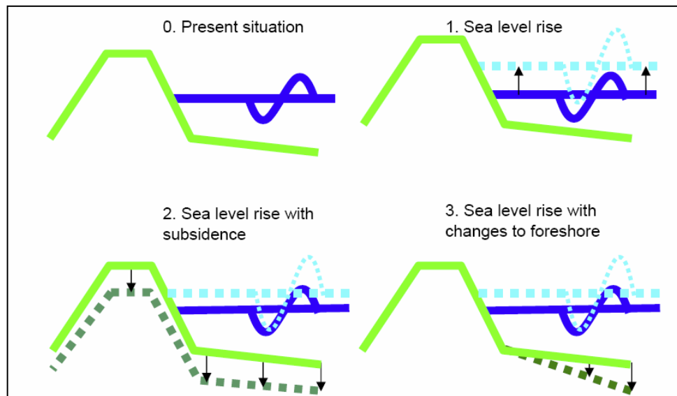
Figure E-1. Potential load cases on FDR elements under sea level rise. Relative sea level change can alter forcings on FDR infrastructure in various ways, depending on the interactions of subsidence and eustatic changes
