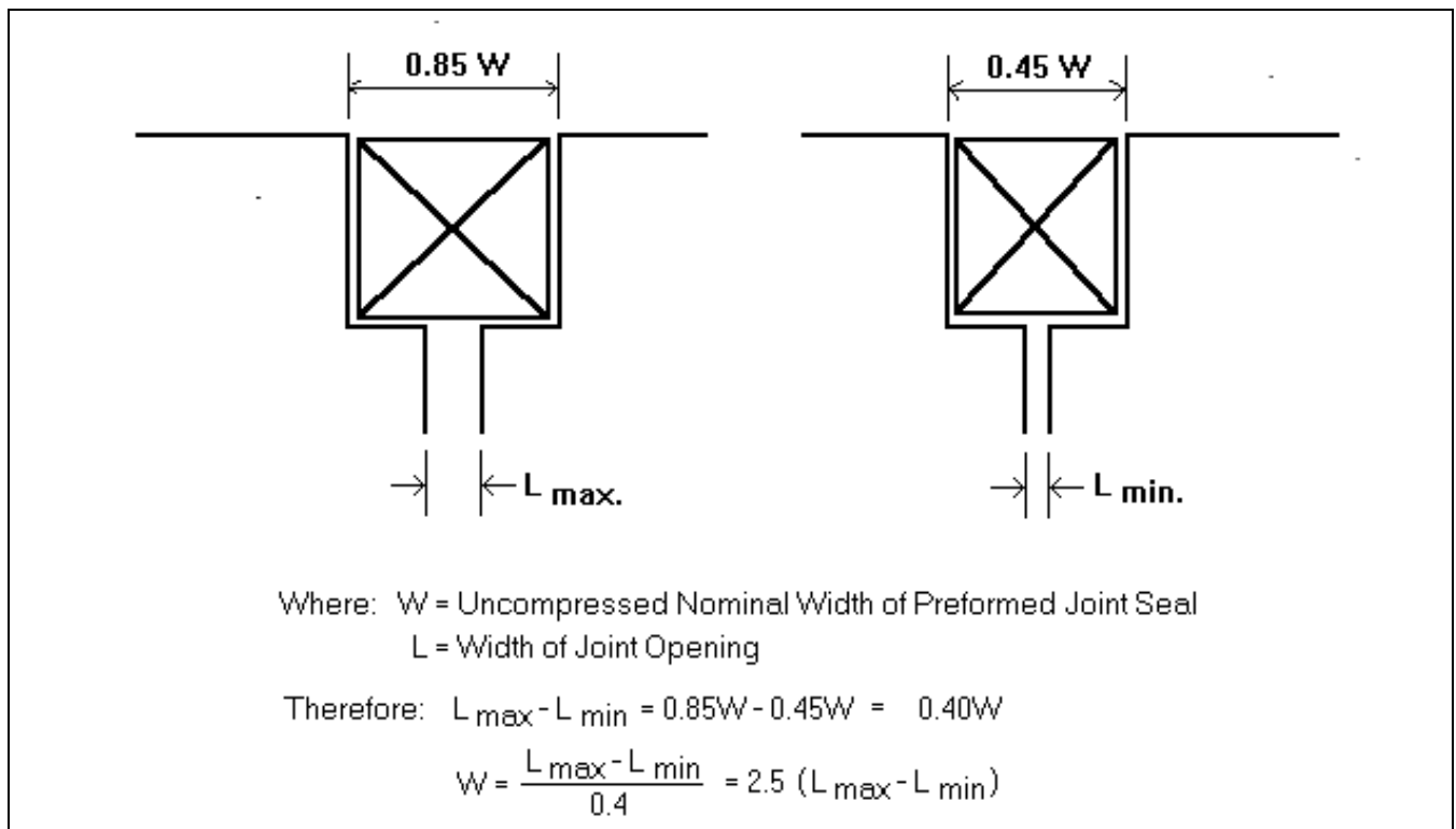
Figure 4-3. Determination of minimum size of compression seal
