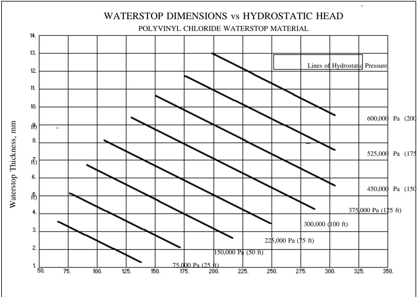
Figure 4-1. This graph shows the general relationship between polyvinyl chloride waterstop dimensions to the hydrostatic head pressure of water
