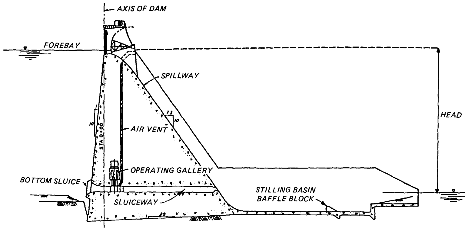
Figure 2-3. Illustration of bottom withdrawal structure, spillway, and stilling basin
