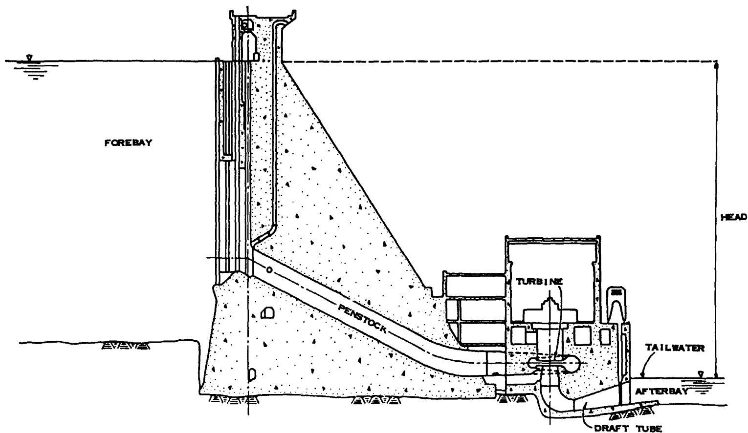
Figure 2-19. Schematic of a hydropower facility
