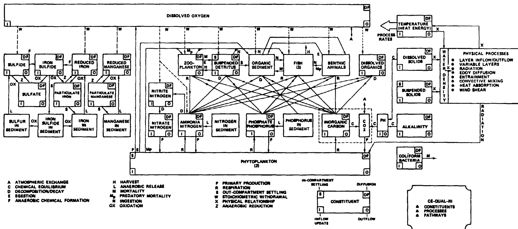
Figure 4-4. Typical water quality model constituents and pathways (from CE-QUAL-R1, Ref. 10)
