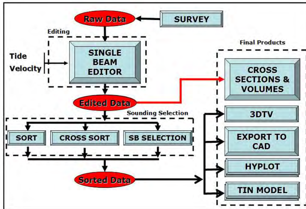
Figure 4-17. Single beam editor data processing flow. Depth sorting options are dependent on final use of the data (plots, volumes, TIN, etc. (HYPACK 2011)
