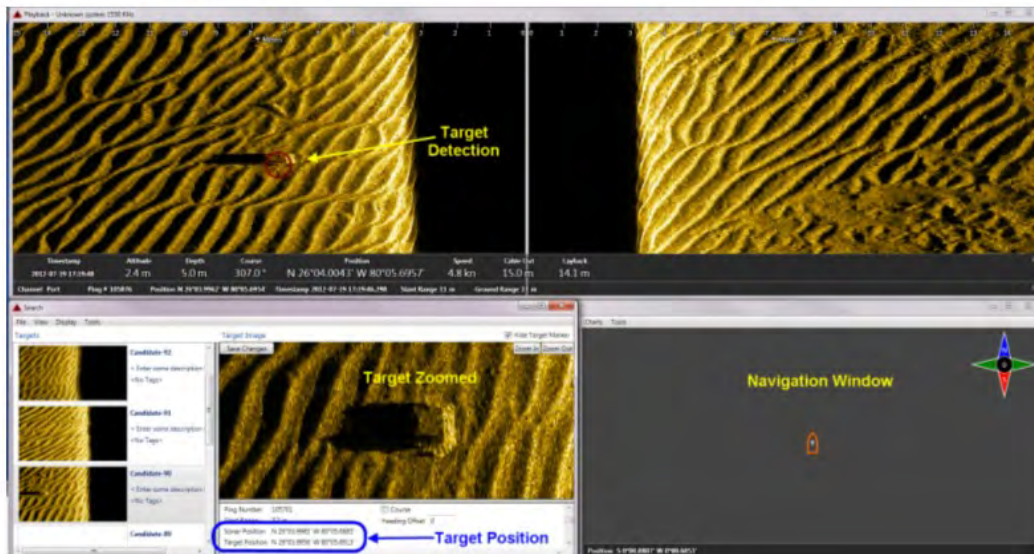
Figure Q-7. Target position calculated by software layback algorithm. (EdgeTech Discover II software)
