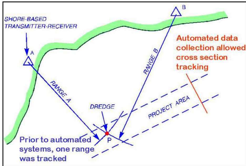
Figure G-16. Range-Range intersection.
