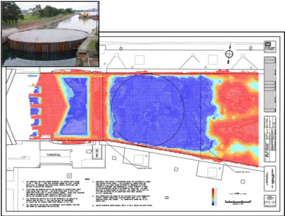
Figure N-9. New Soo Lock—Multibeam survey of cofferdam excavation. Soo Area Office. (Detroit District)
