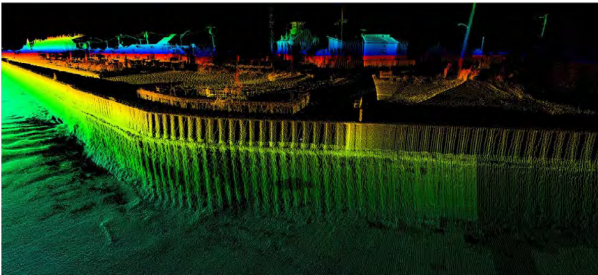
Figure 11-22. Combined vessel mounted mobile laser scanner with multibeam hydrographic surveys of sheet piling structure – Manasquan Inlet, NJ (Philadelphia District).
