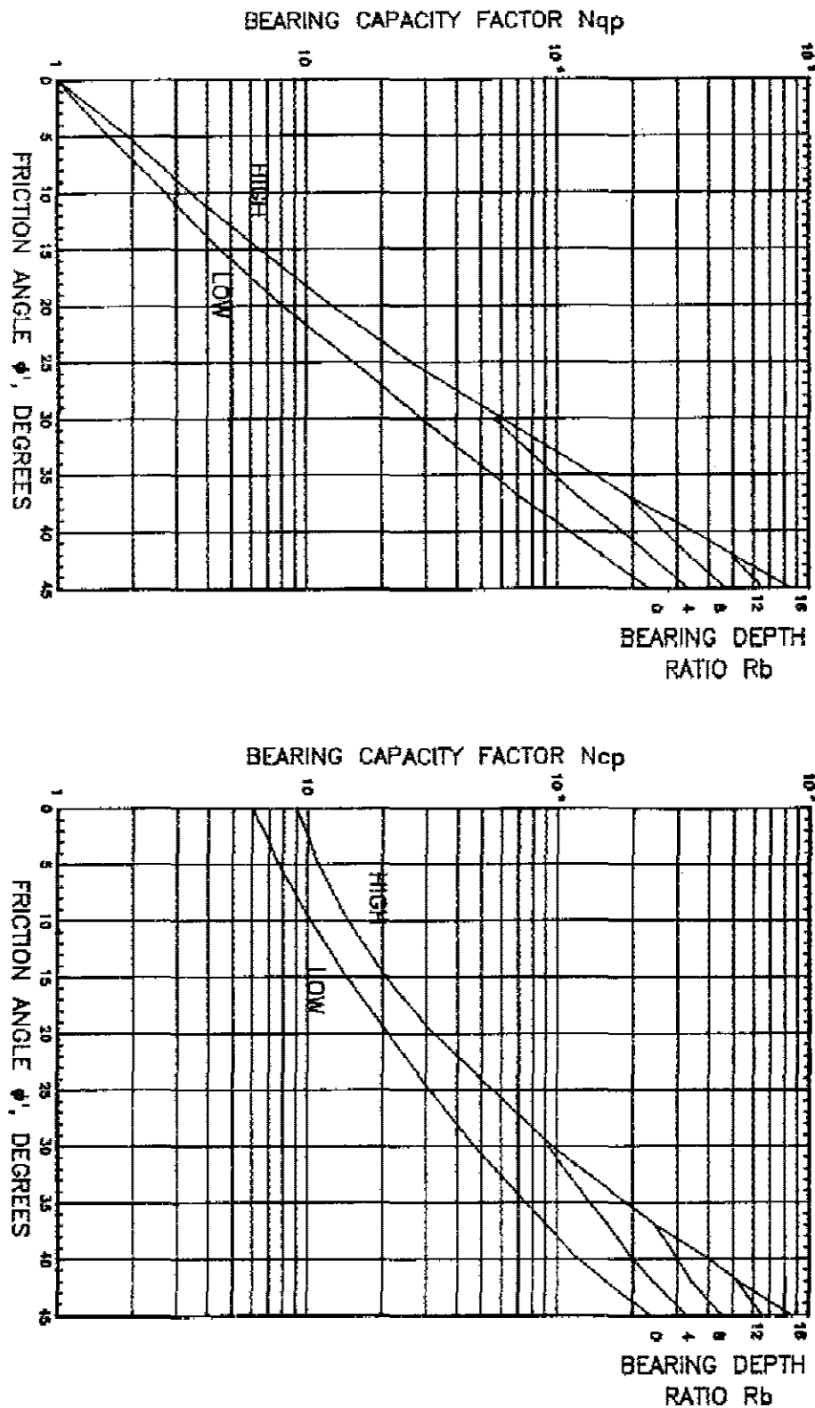
Figure 5-15. Bearing capacity factors for Meyerhof method (Data from Meyerhof 1976)
