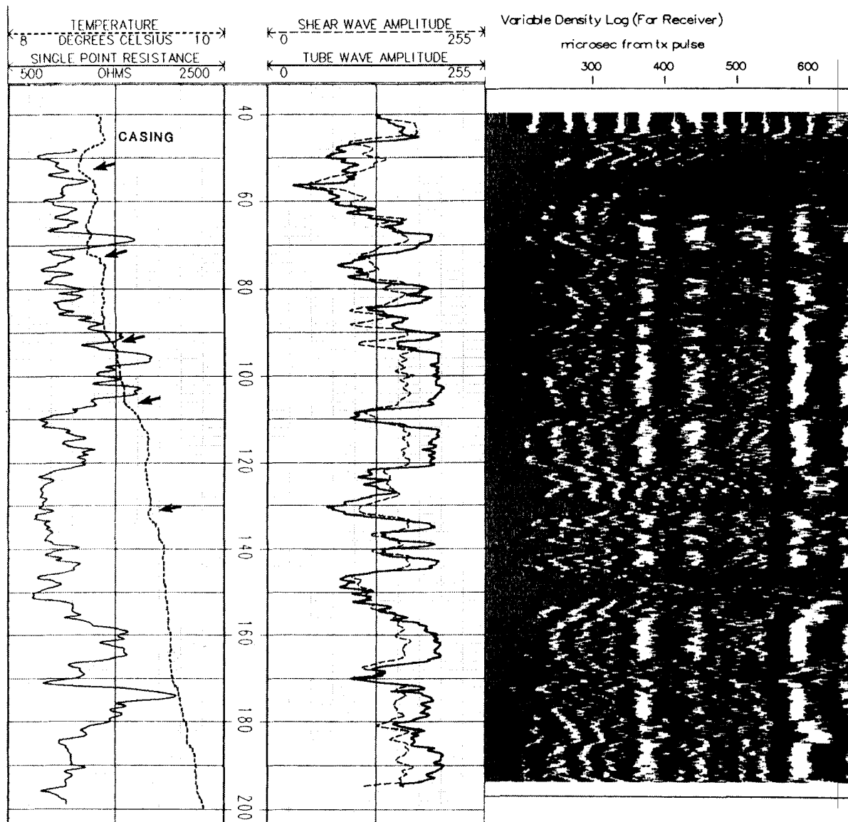
Figure 7-27. Composite of logs showing the location of permeable fractures indicated by the arrows at changes in temperature gradient and by low tube and shear wave amplitude (Yearsley and Crowder 1990; copyright permission granted by Colog, Inc.)
