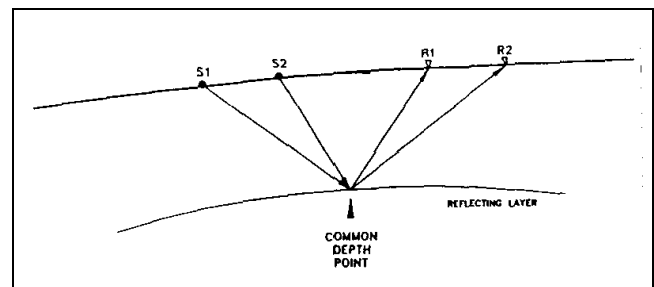
Figure 3-30. Illustration of common-depth point recording
