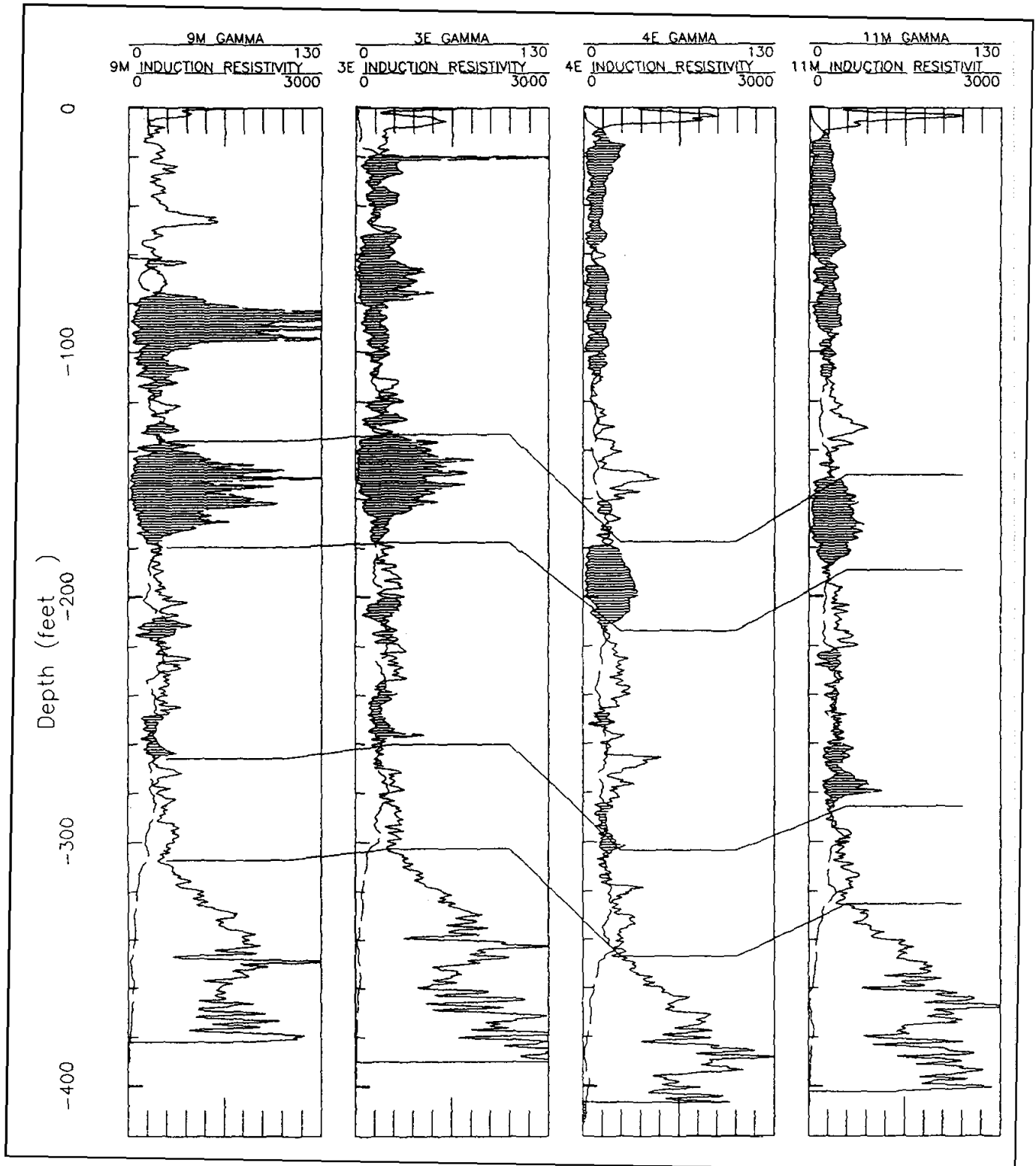
Figure 7-2. Cross section of four test holes in the Chicago area showing correlation enhanced by computer shading between gamma and induction logs
