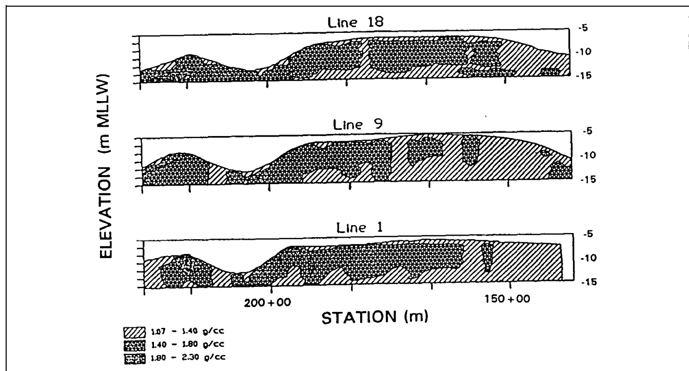
Figure 3-38. Density cross sections in Gulfport Ship Channel, Mississippi (Ballard, McGee, and Whalin 1992)
