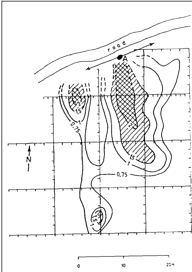
Figure 4-24. Network of SRP-IP profiles with the contours of IP values \eta_p (percent) and the extent of the contaminant interpreted on the basis of the geophysical survey; location A is the known outcrop of the slag-type contaminant and the position of the VES-IP measurement (Cahyna, Mazac, and Vendhodova 1990; copyright permission granted by Society of Exploration Geophysicists)
