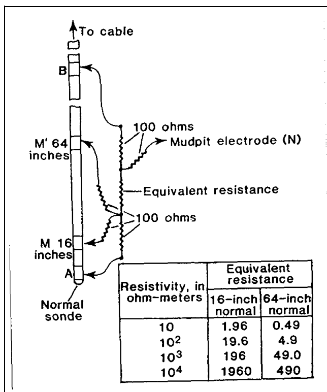
Figure 7-14. System for calibrating normal-resistivity equipment
