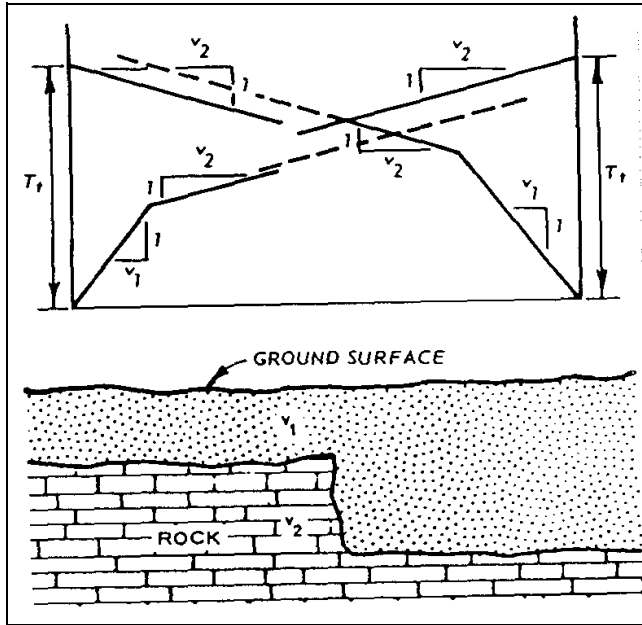
Figure 3-21. Subsurface cliff
