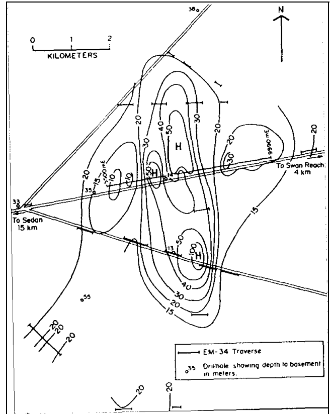
Figure 4-48. Apparent resistivity contours in \Omega\text{m} from a terrain conductivity meter in southern Australia (Dodds and Ivic 1990; copyright permission granted by Society of Exploration Geophysicists)
