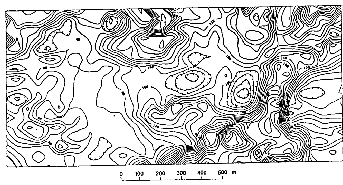
Figure 4-45. Contours of apparent conductivity measured with ground conductivity meter over dry farm land, Alberta, Canada (Wood (1987) in McNeill (1990); copyright permission granted by Society of Exploration Geophysicists)
