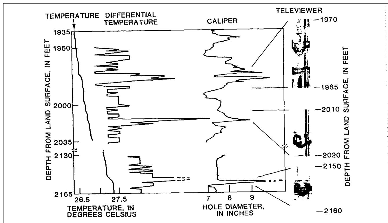
Figure 7-35. Temperature, differential-temperature, caliper, and acoustic-televviewer logs of Sears test well No. 1, near Raleigh, NC
