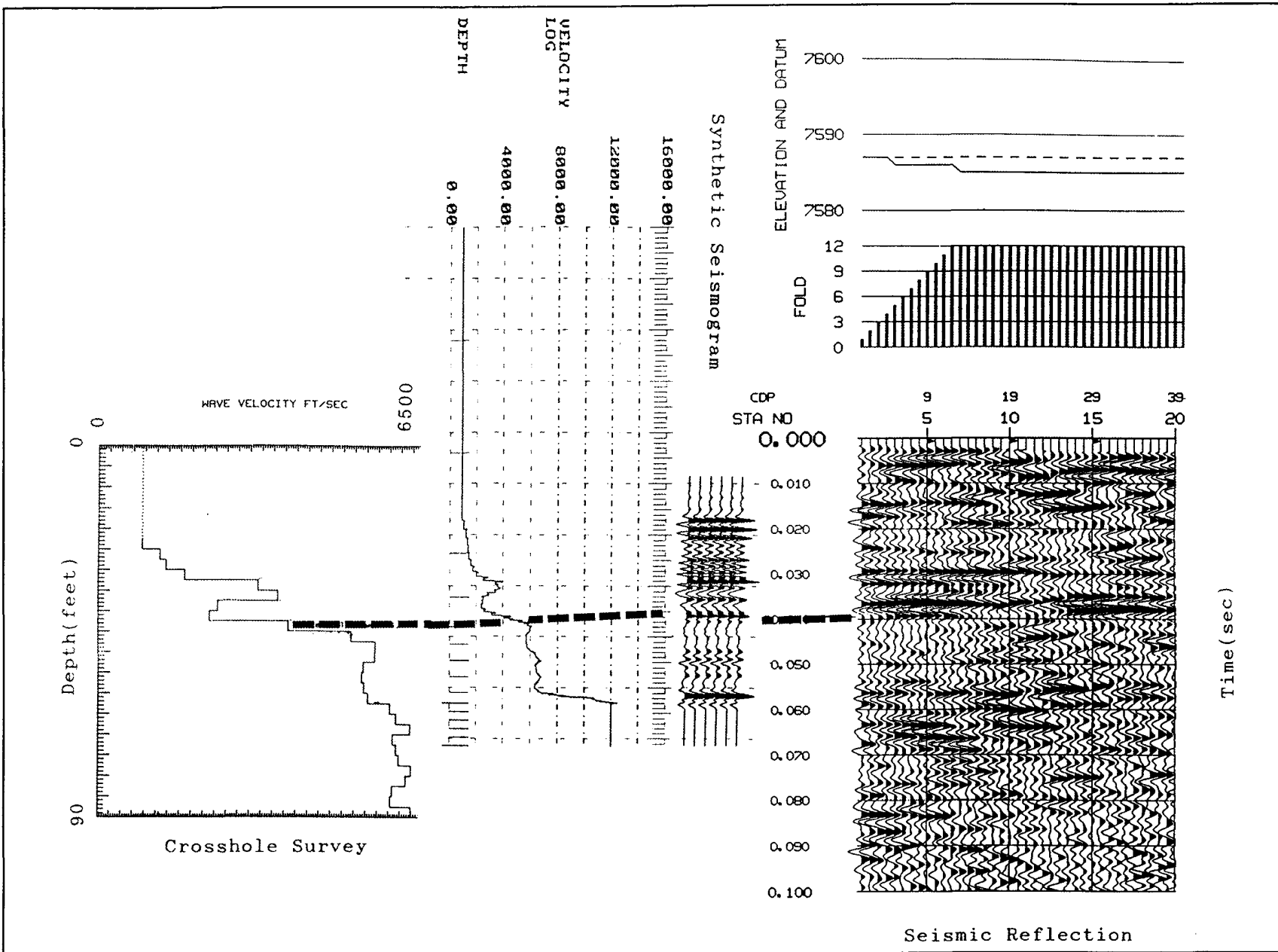
Figure 7-49. Correlation between crosshole survey, velocity log, synthetic seismogram and surface seismic reflection section
