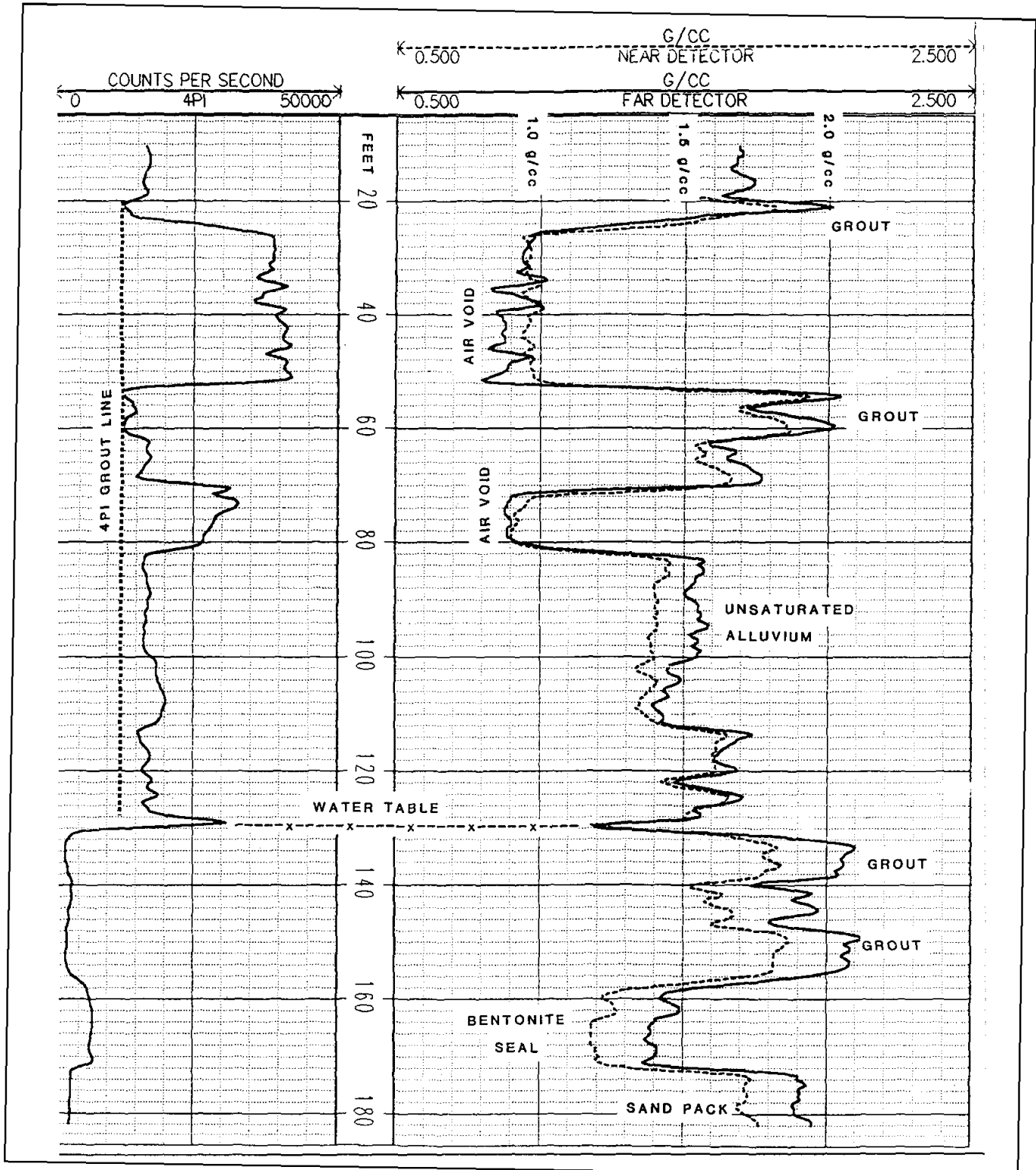
Figure 7-43. Dual-spaced and "4π" density logs in a cased monitoring well showing completion as interpreted from the logs (Yearsley, Crowder, and Irons 1991; copyright permission granted by Colog, Inc.)
