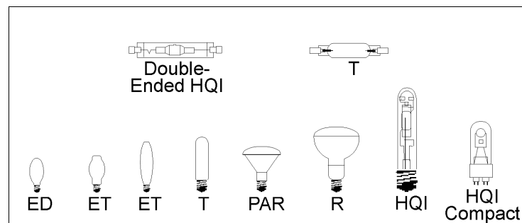
Fig. 27 Standard HID lamp types
