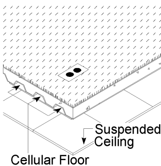
Fig. 22 Cellular floor distribution
