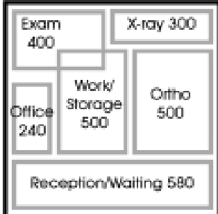
Fig. 2 Blocking Diagram
