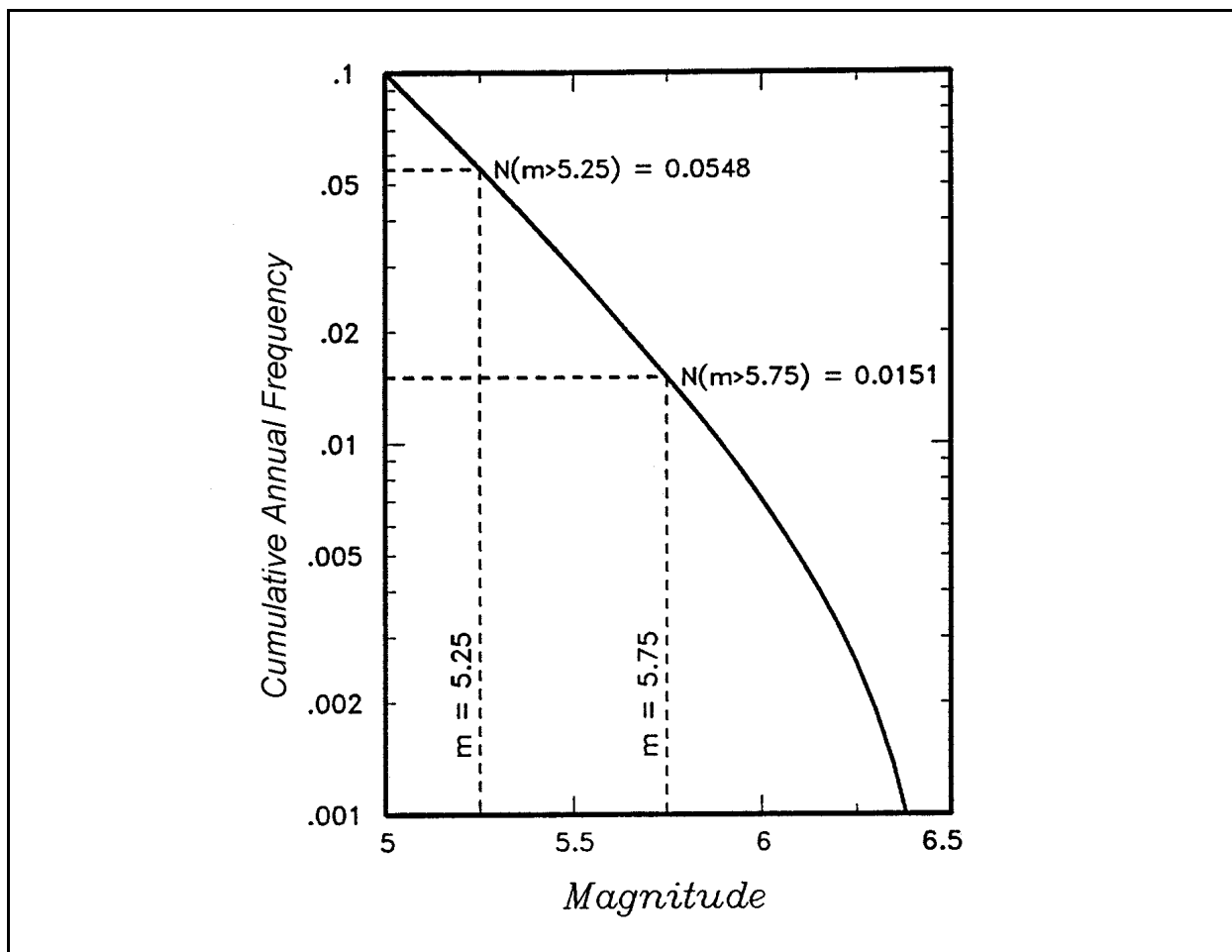
Figure G1-2. Example recurrence rate calculation
