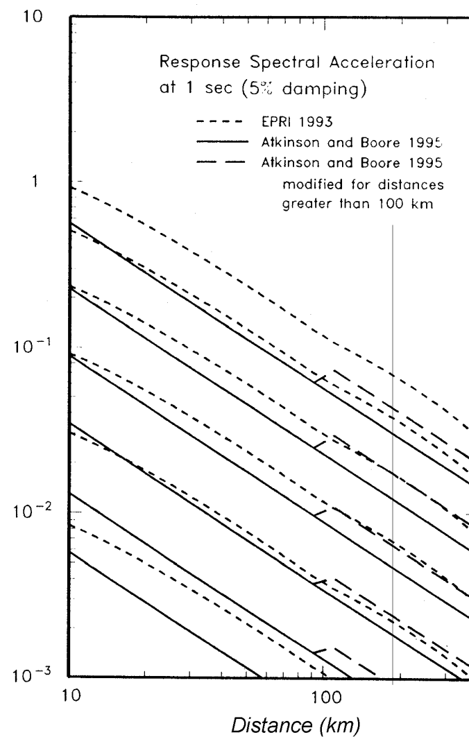
Figure G4-4. Attenuation curves of Atkinson and Boore (1995) and EPRI (1993) for peak ground acceleration and response spectral acceleration at 1.0-sec period. Note: Lowest curve for each relationship is for m_b 5.0; highest curve, for m_b 7.5
