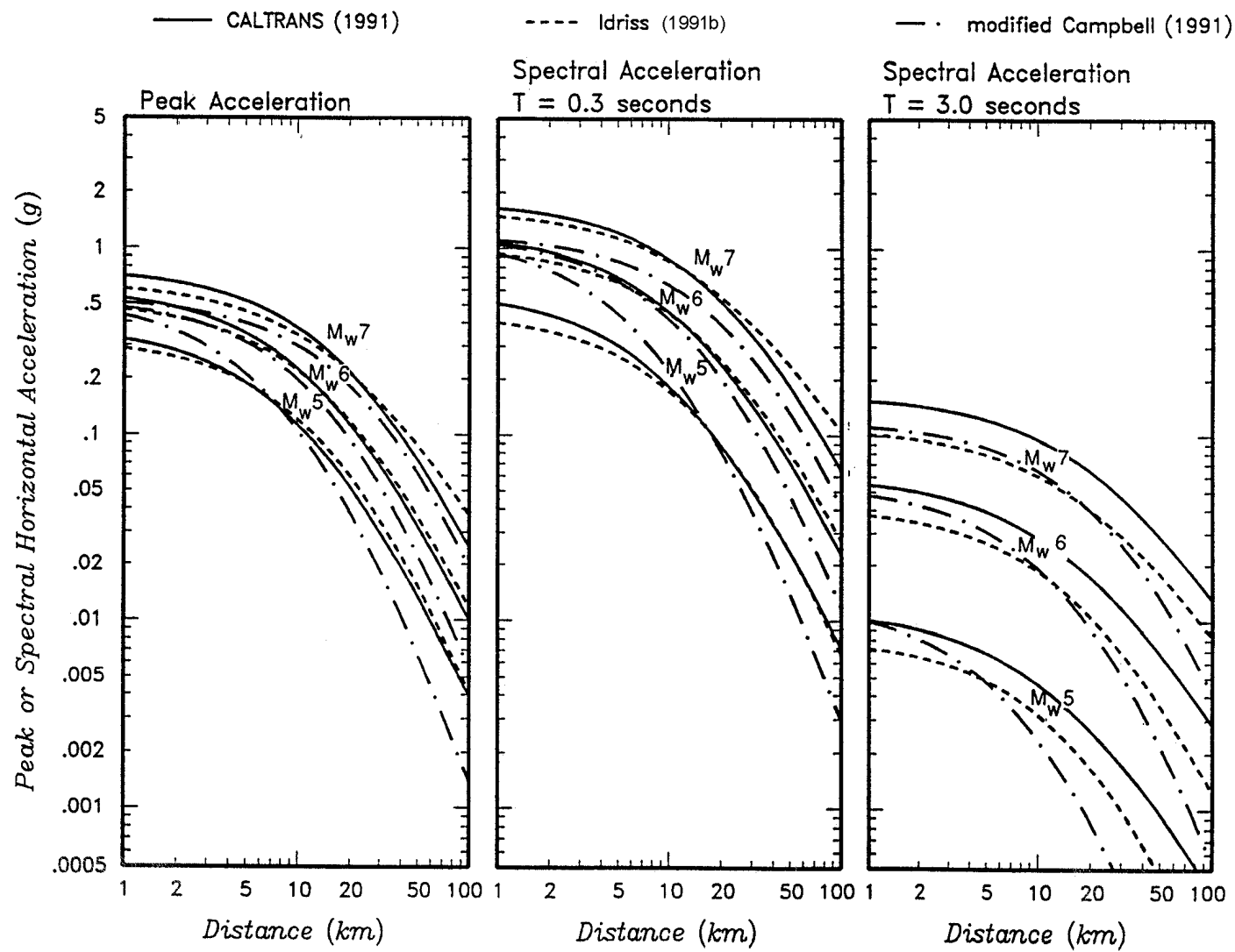
Figure G2-7. Ground motion attenuation relationships
