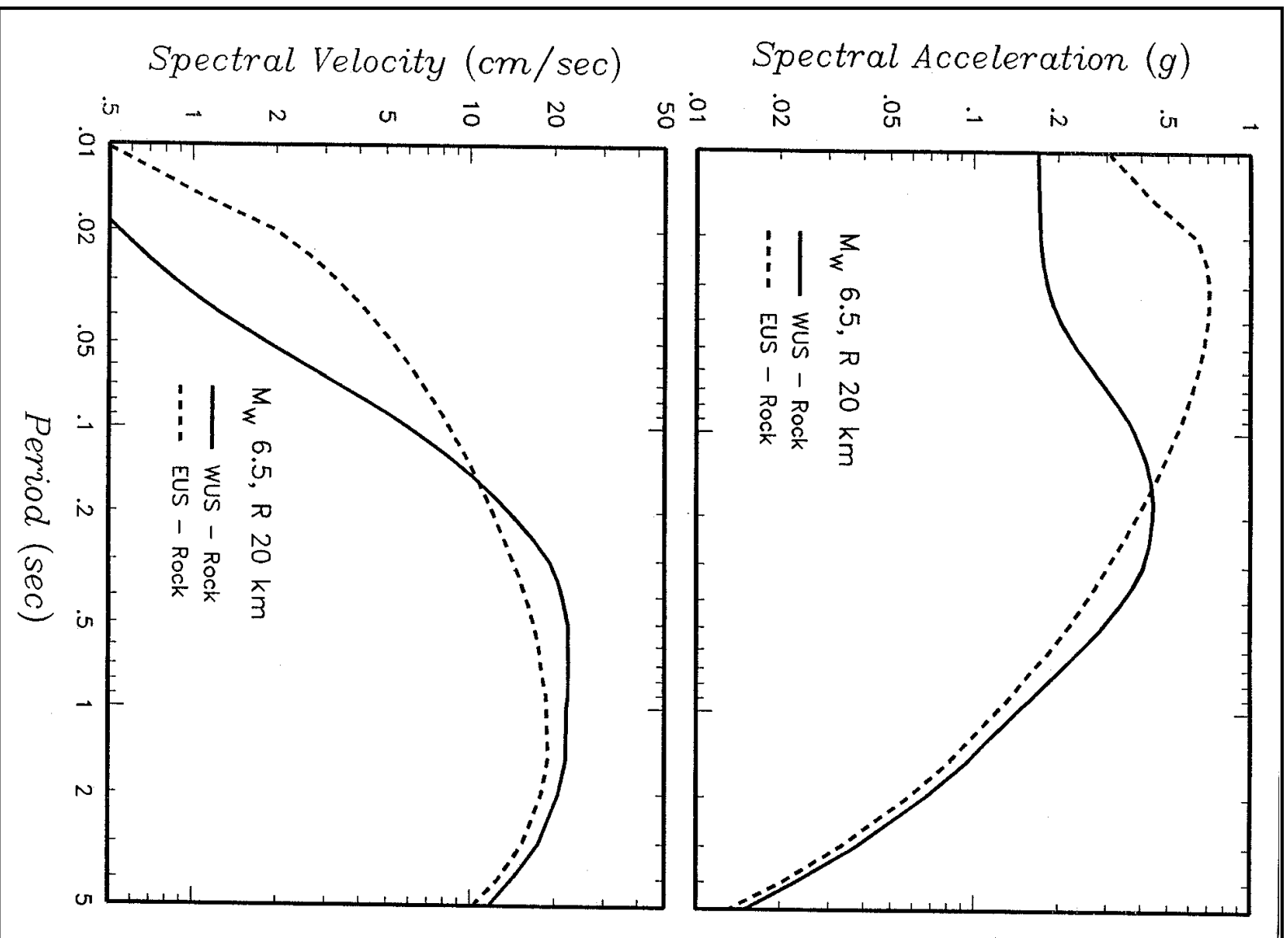
Figure 3-13. Comparison of response spectra for a magnitude 6.5 earthquake at 20 km using WUS and EUS attenuation relationships (calculated using BLWN/RVT model as formulated by Silva and Green 1989)
