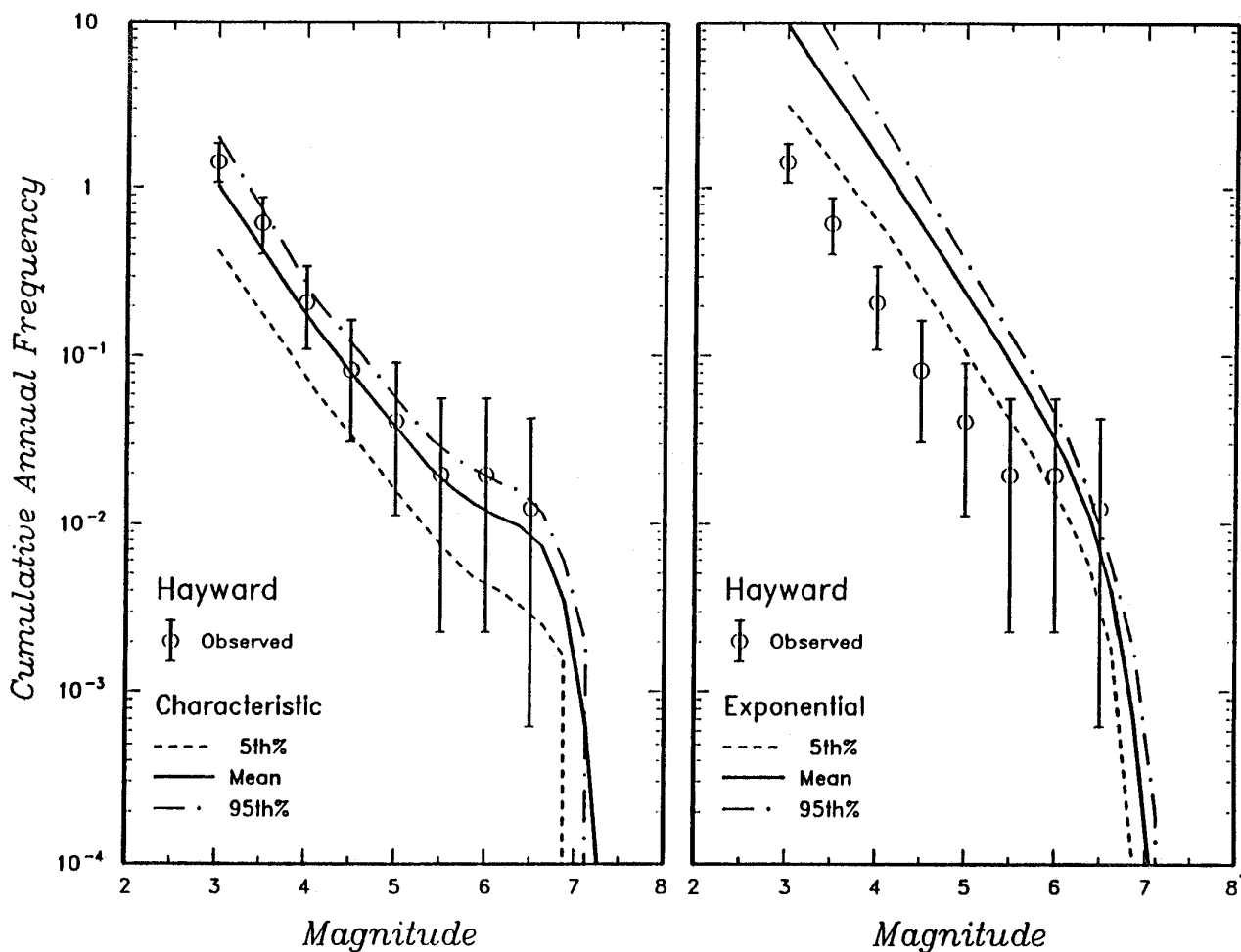
Figure G2-4. Comparison of recurrence rates developed from independent seismicity and from fault slip rates for the Hayward fault. Predicted recurrence rates are shown for the characteristic earthquake and exponential magnitude distribution models
