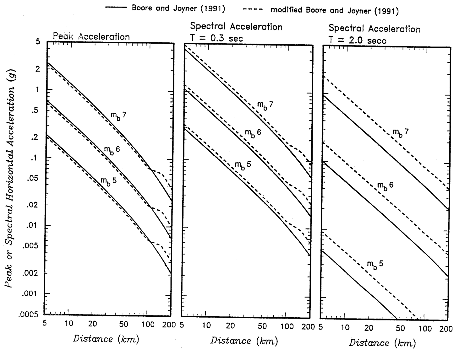
Figure G3-6. Attenuation relationships
