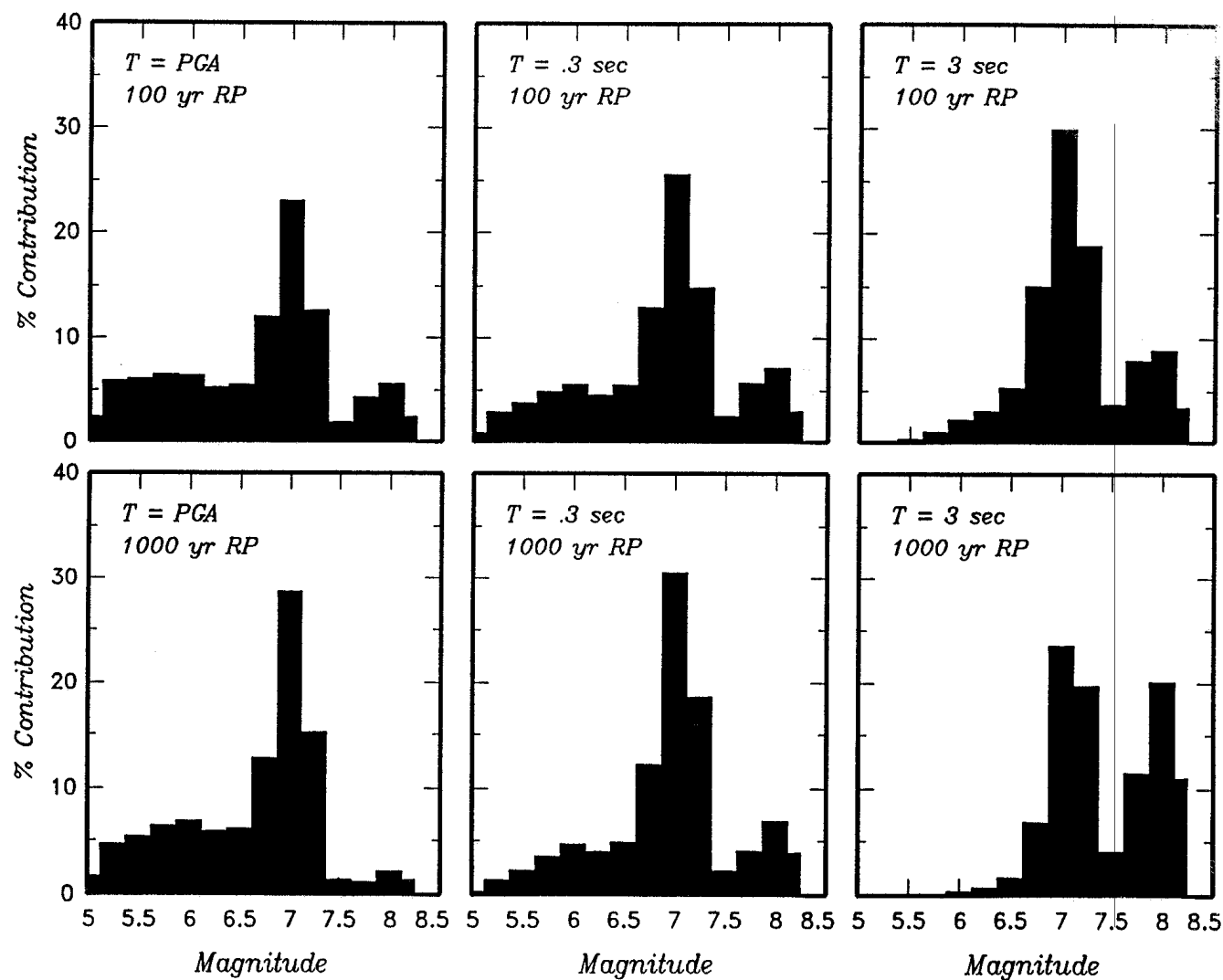
Figure G2-10. Contributions of events in various magnitude intervals to the mean hazard at the site. Shown are results for peak acceleration and 5 percent-damped spectral accelerations at periods of 0.3 and 3.0 sec
