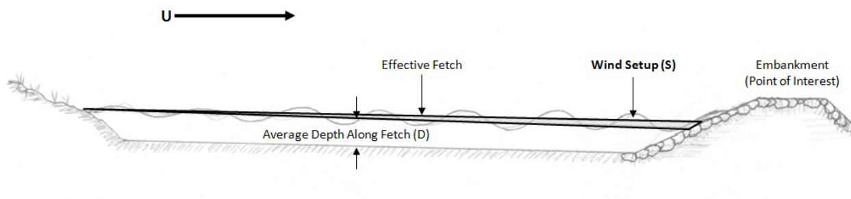
Figure C-6. Wind Setup.
