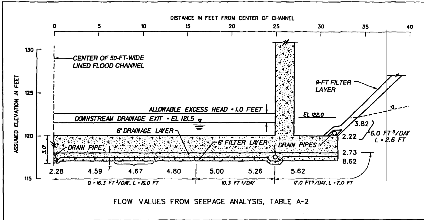
Figure C-7. Flows into drainage blanket from analysis of U-frame channel section
