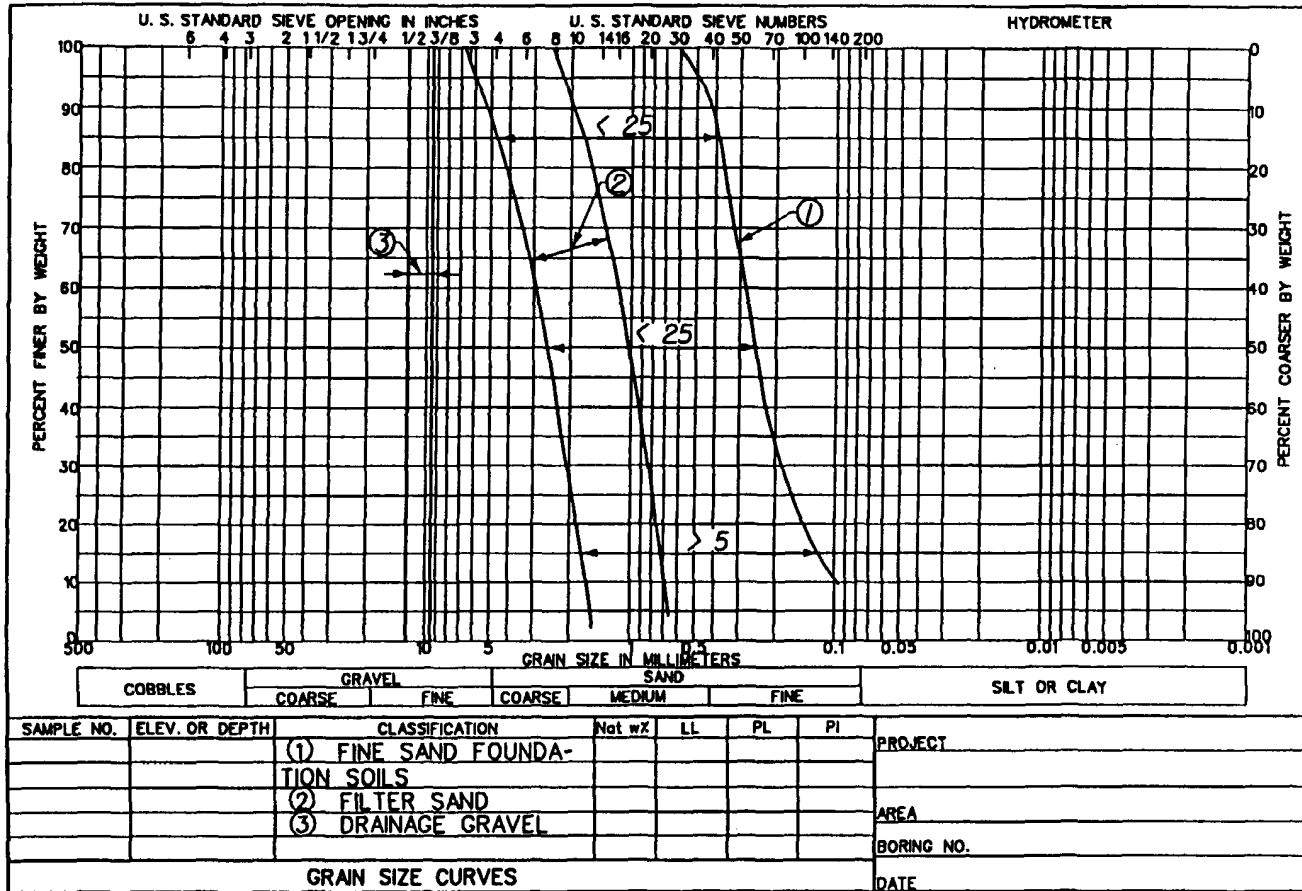
Figure C-12. Gradation of drainage materials for trapezoidal channel section
