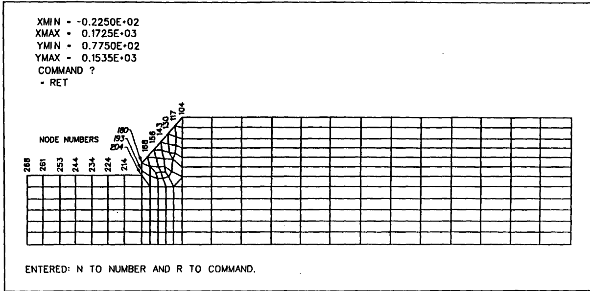
Figure C-3. Finite element grid used for analysis of U-frame channel section
