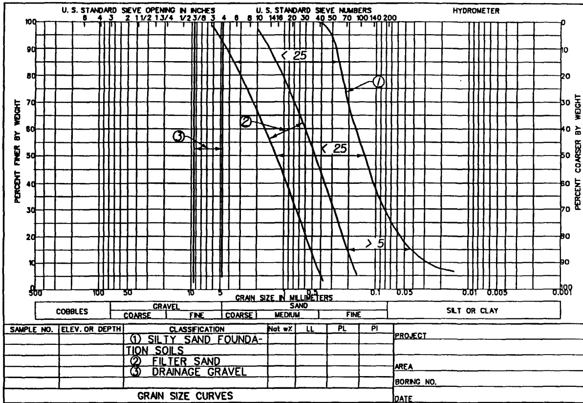
Figure C-8. Gradation of drainage materials for U-frame channel section
