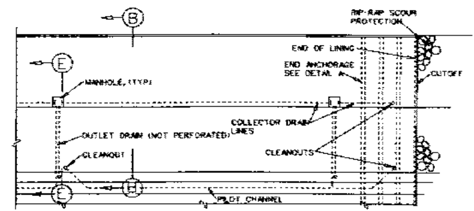
CHANNEL WITH PILOT CHANNEL NO SCALE
