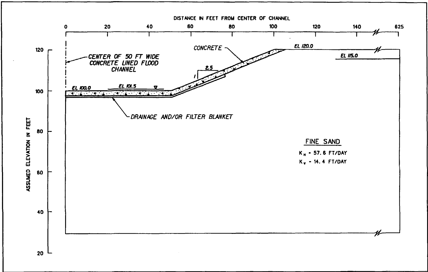
Figure C-10. Example trapezoidal channel and foundation conditions
