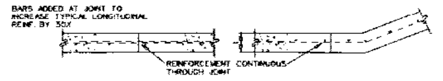
TRANSVERSE CONSTRUCTION JOINT LONGITUDINAL
