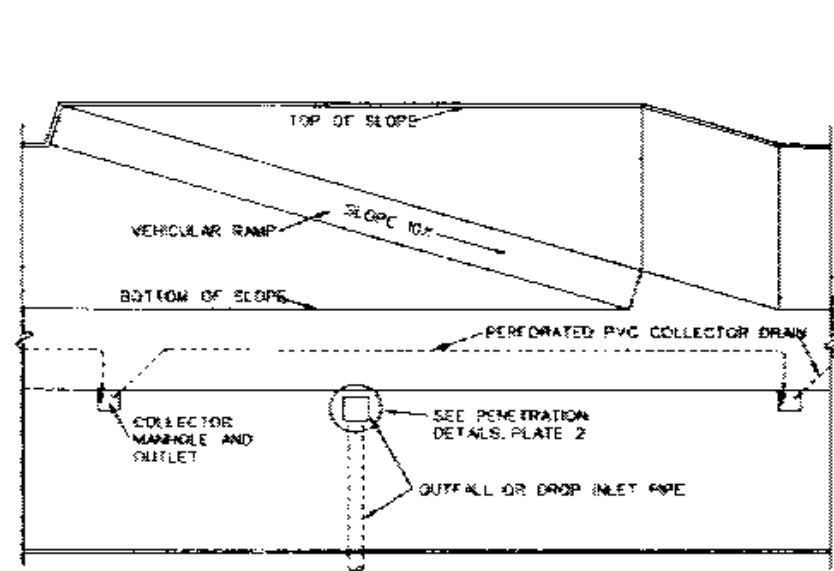
CHANNEL WITH ONE DRAIN LINE NO SCALE
