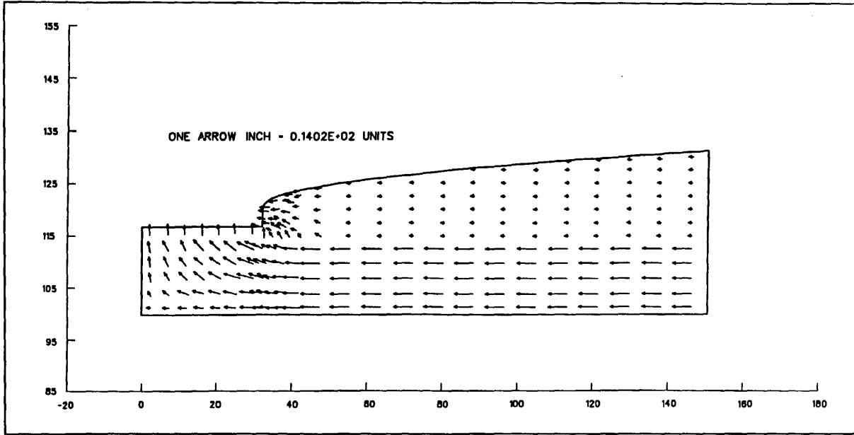
Figure C-5. Vector diagram of flow from analysis of U-frame channel section
