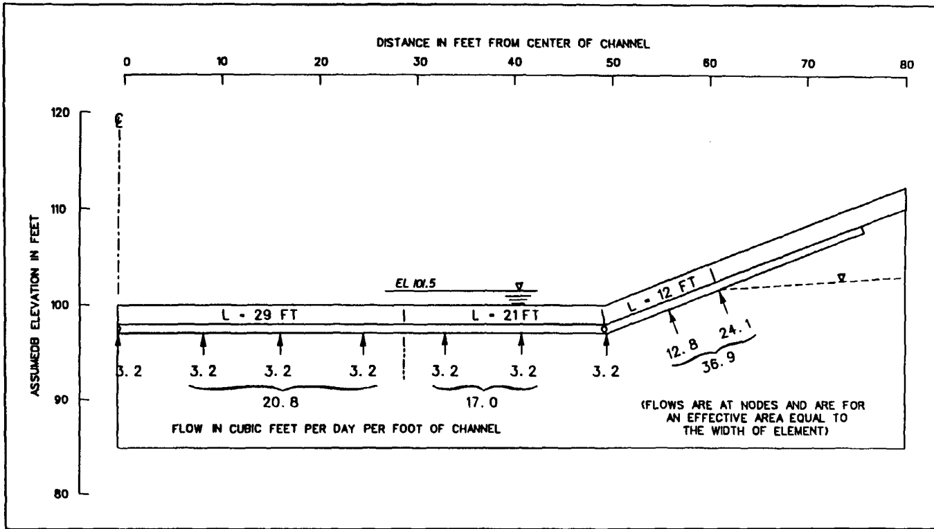
Figure C-11. Flows into drainage blanket from analysis of trapezoidal channel section
