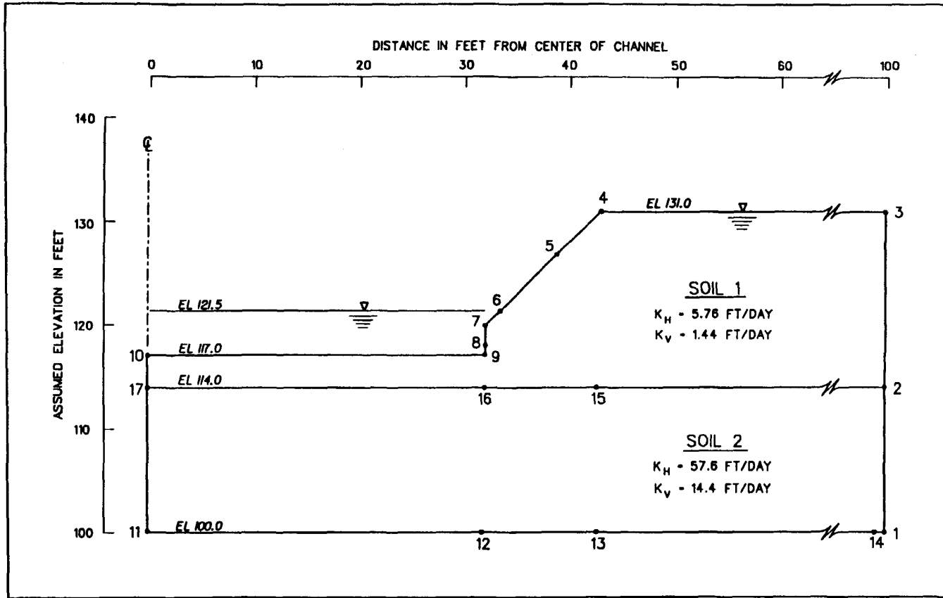
Figure C-2. Profile utilized in developing data file
