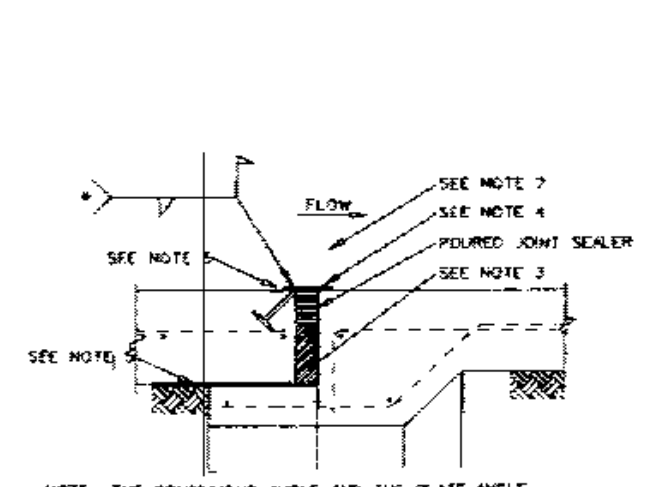
SLAB EXPANSION JOINT DETAIL NO SCALE
