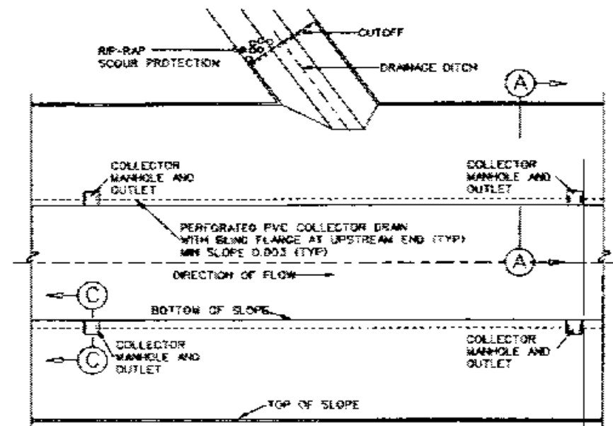
CHANNEL WITH TWO DRAIN LINES NO SCALE
