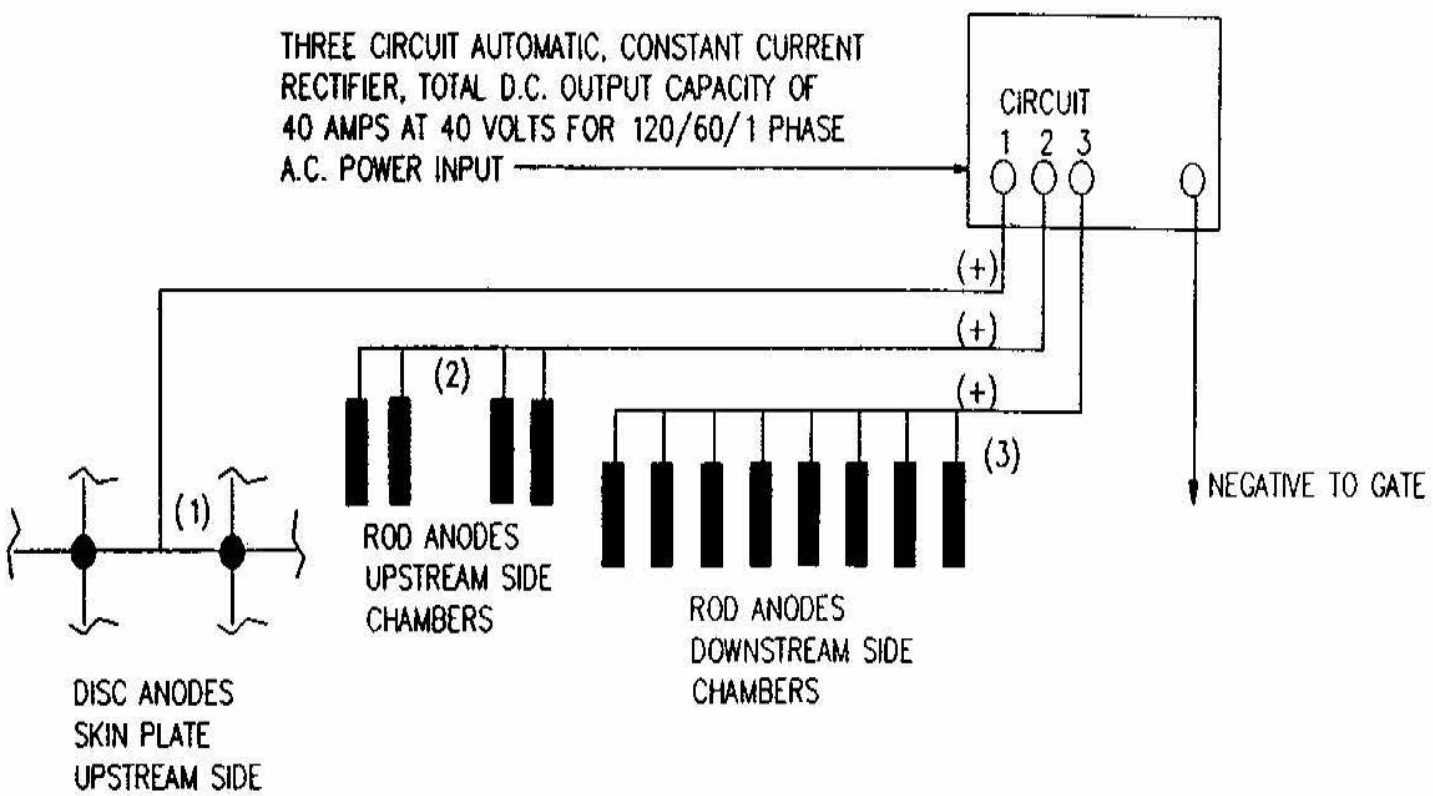
FIGURE B-6. CIRCUIT DIAGRAM FOR LOCK MITER GATE
