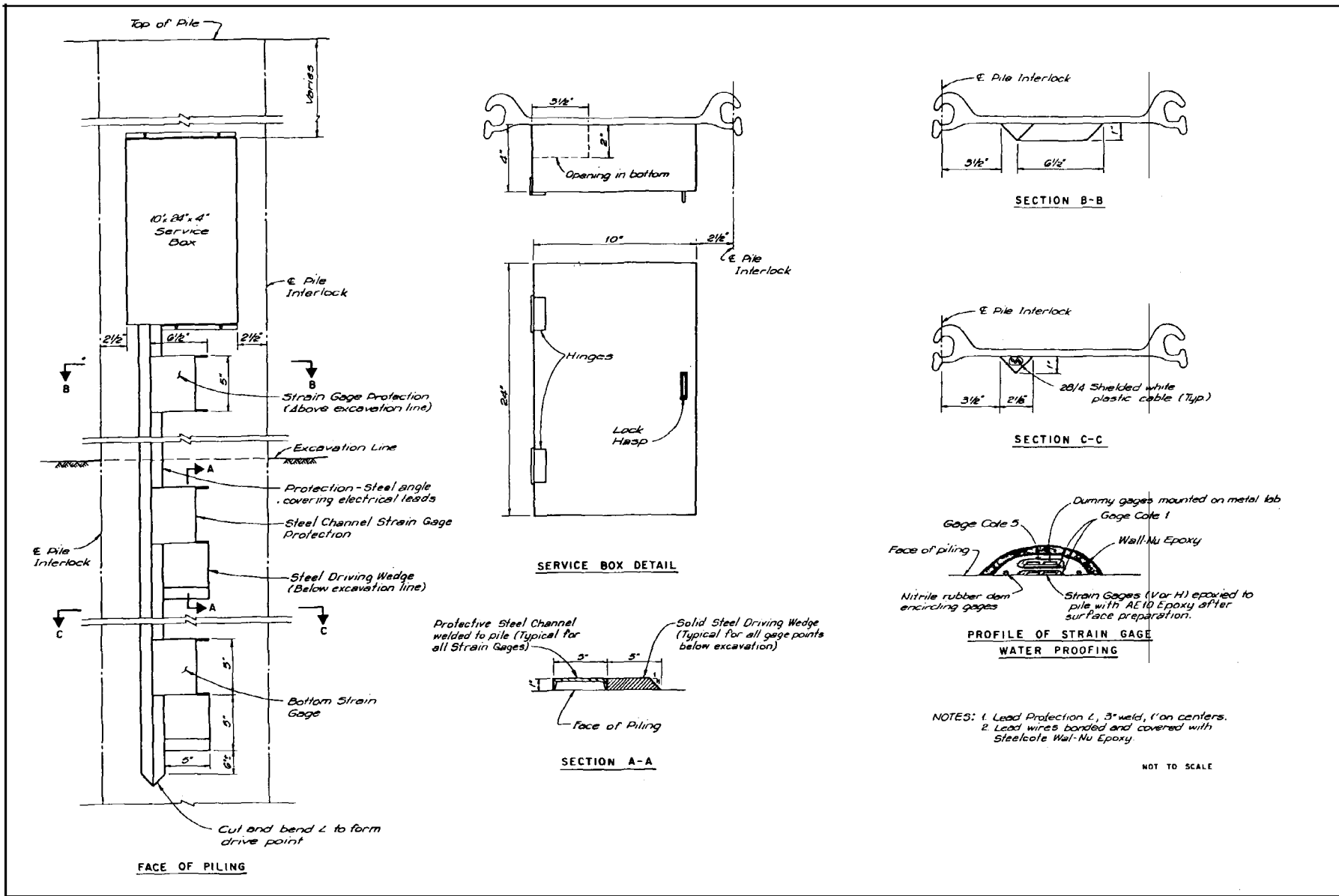
Figure 7-4. Strain gage details
