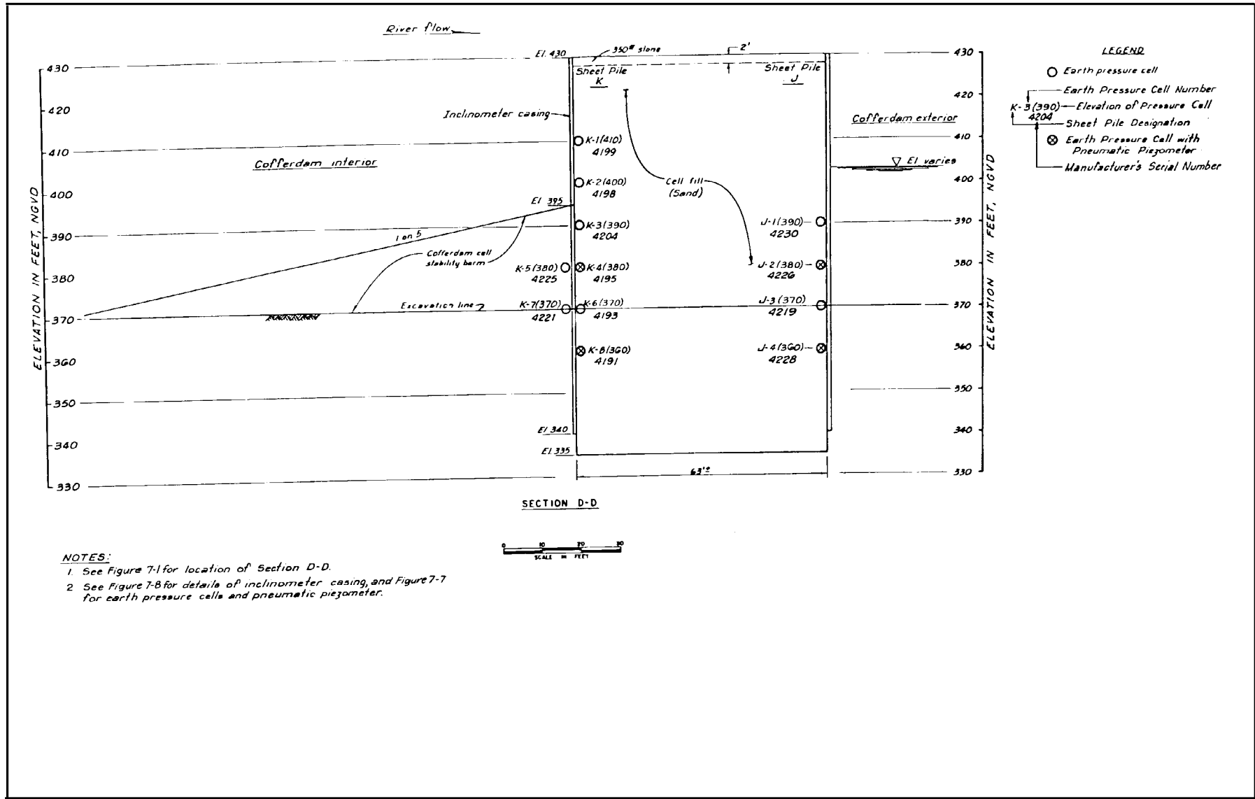
Figure 7-6. Location of earth pressure cells and inclinometers, SECTION D-D
