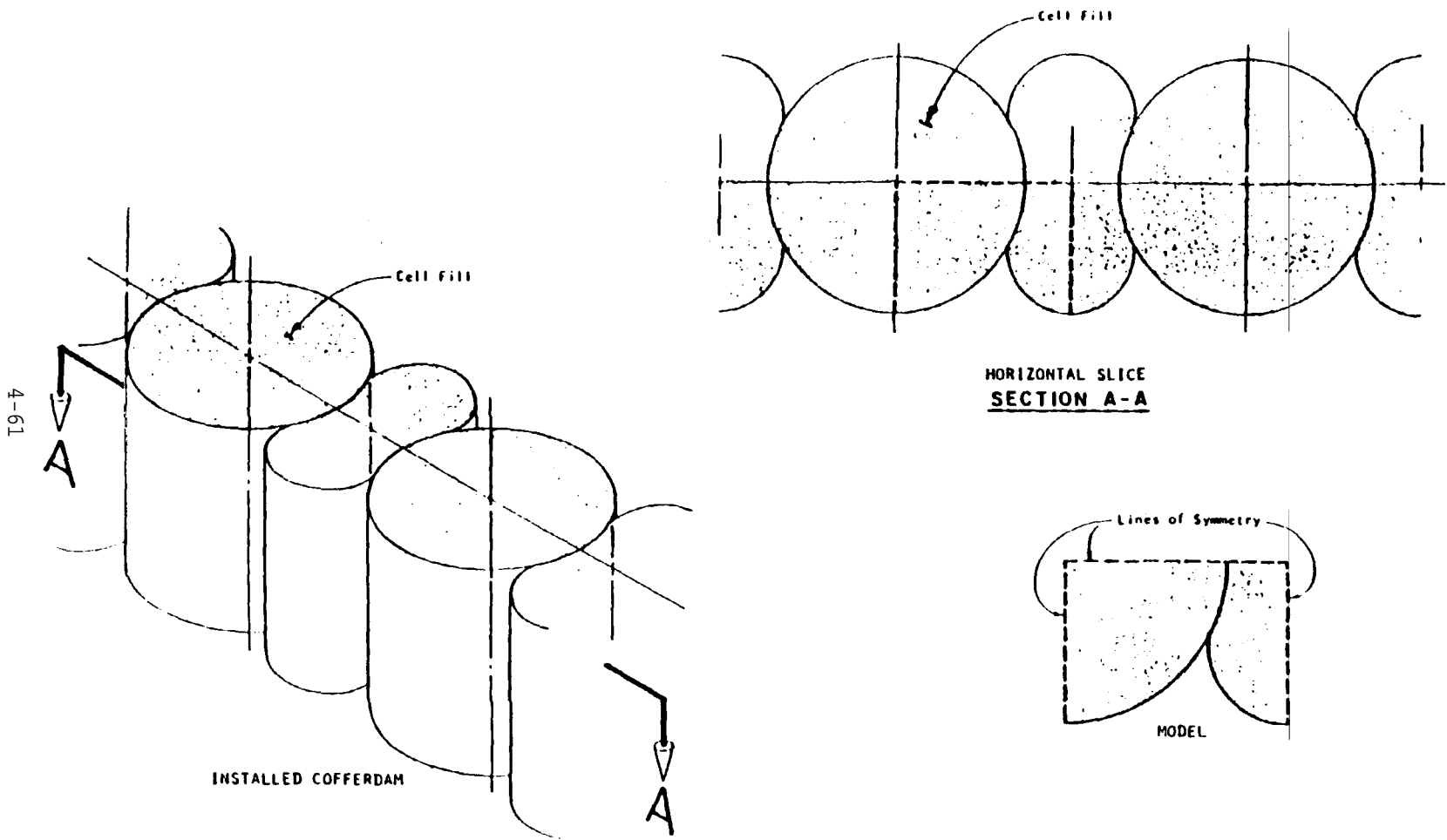
Figure 4-24. Schematic drawing, horizontal slice model
