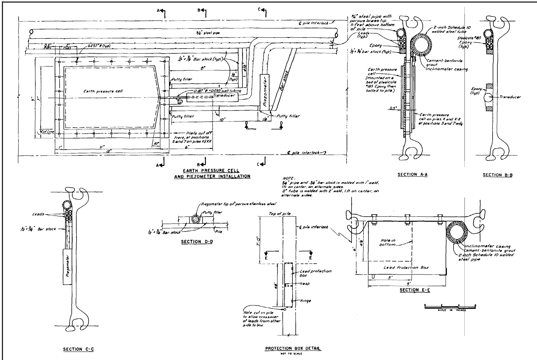
Figure 7-7. Earth pressure cell and piezometer details
