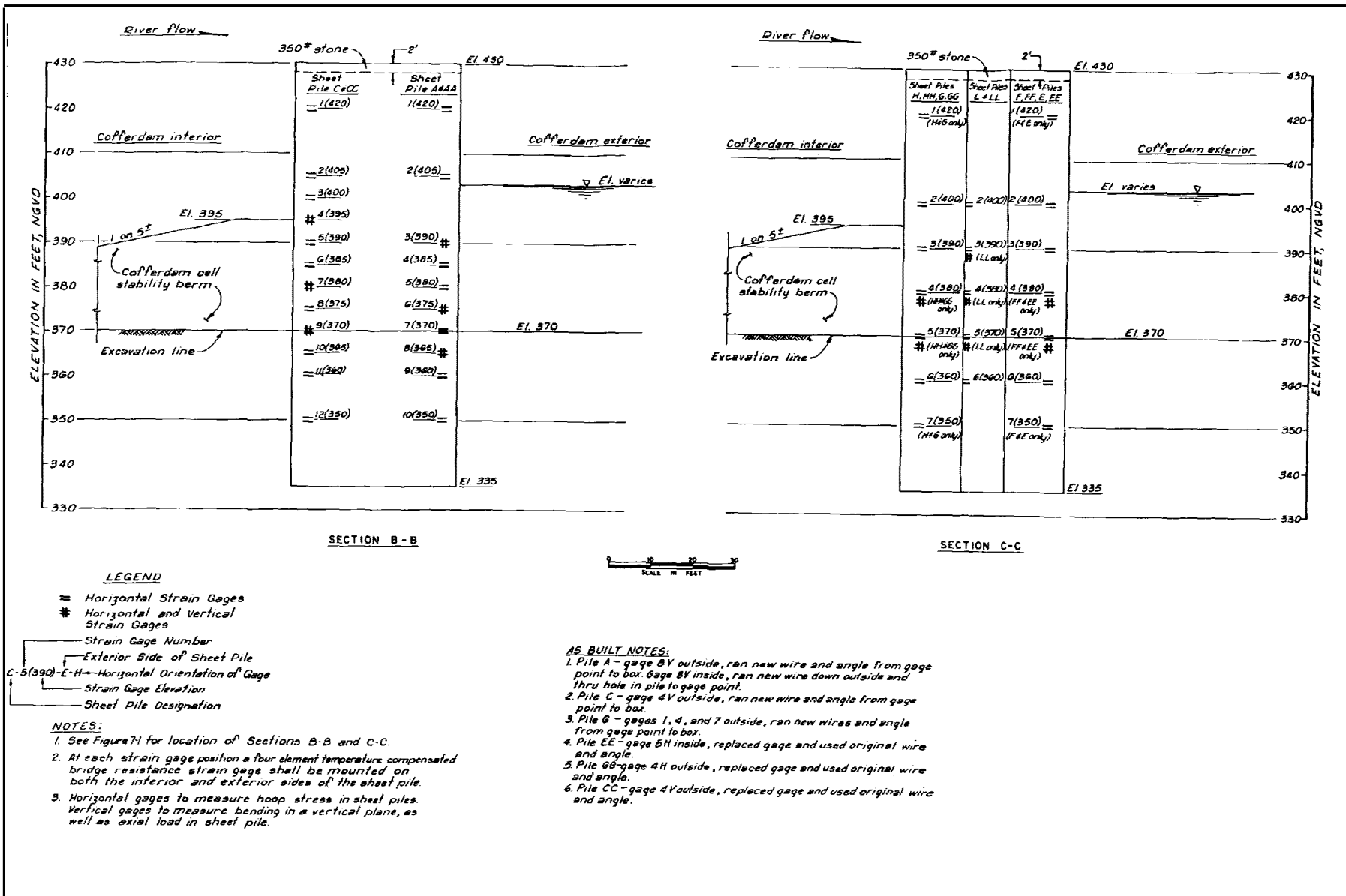
Figure 7-3. Strain gage locations adjacent to wye piles
