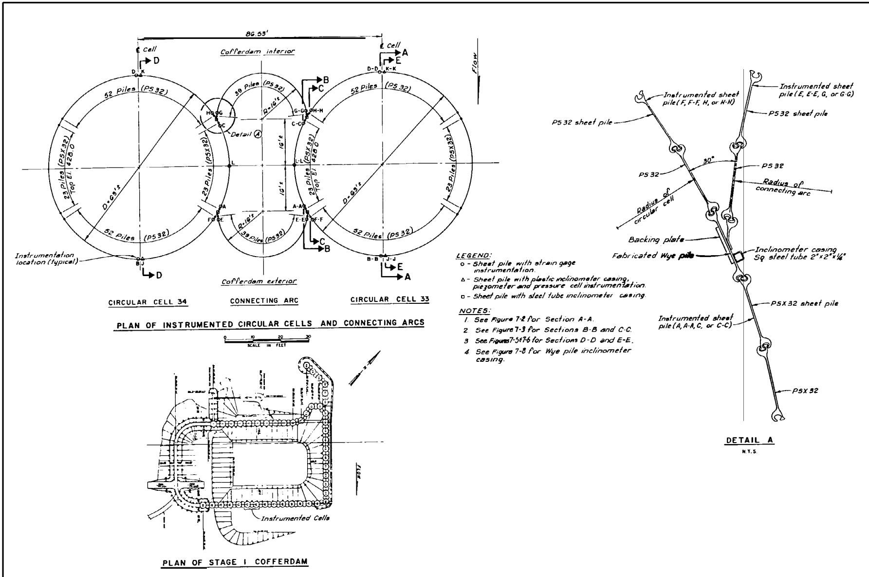
Figure 7-1. Plan of instrumentation
