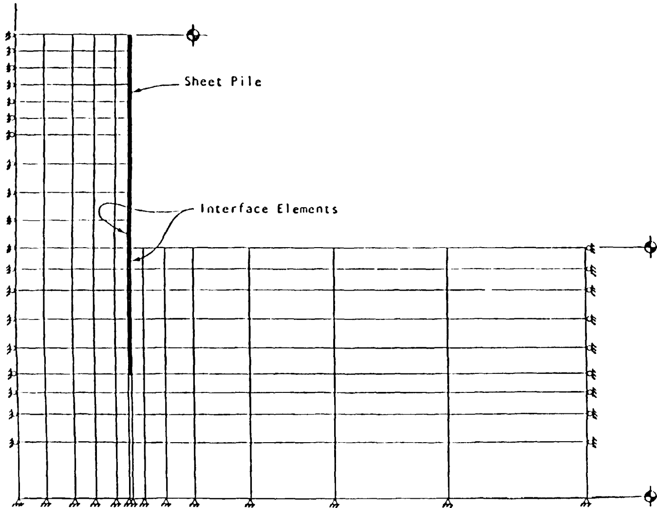
Figure 4-23. Finite element mesh for axisymmetric analyses of main cell filling
