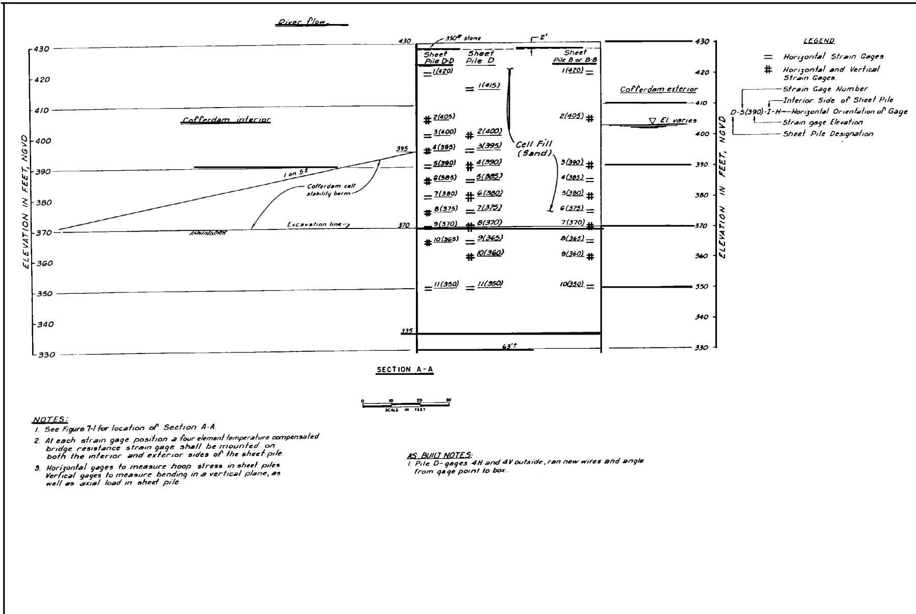
Figure 7-2. Strain gage locations
