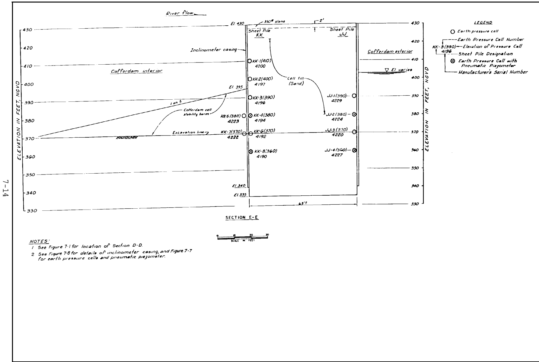
Figure 7-5. Location of earth pressure cells and inclinometers, Section D-D
