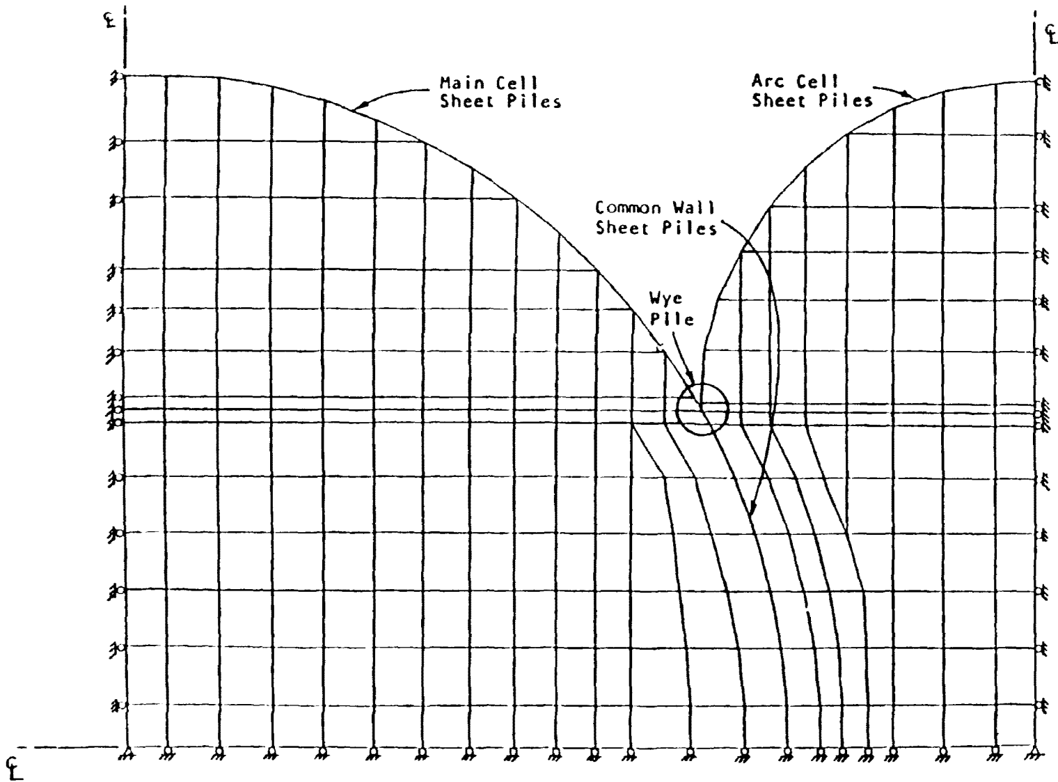
Figure 4-25. Finite element mesh for horizontal slice analysis of cell filling
