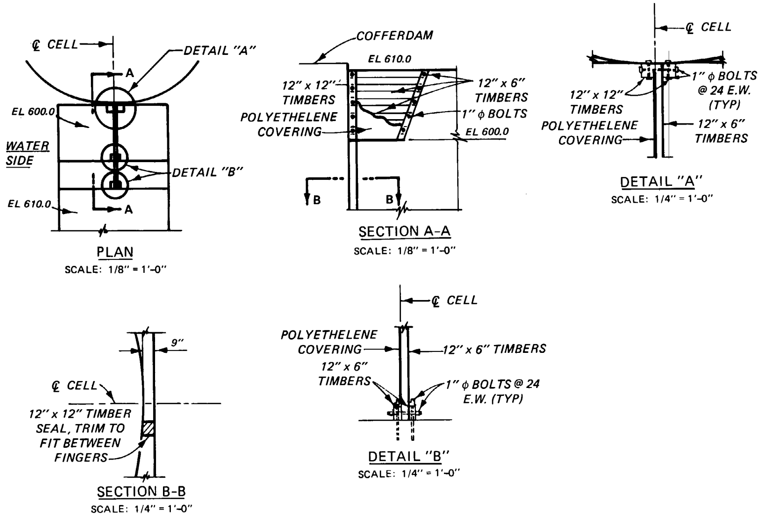
Figure 2-3. Typical tie-in details
