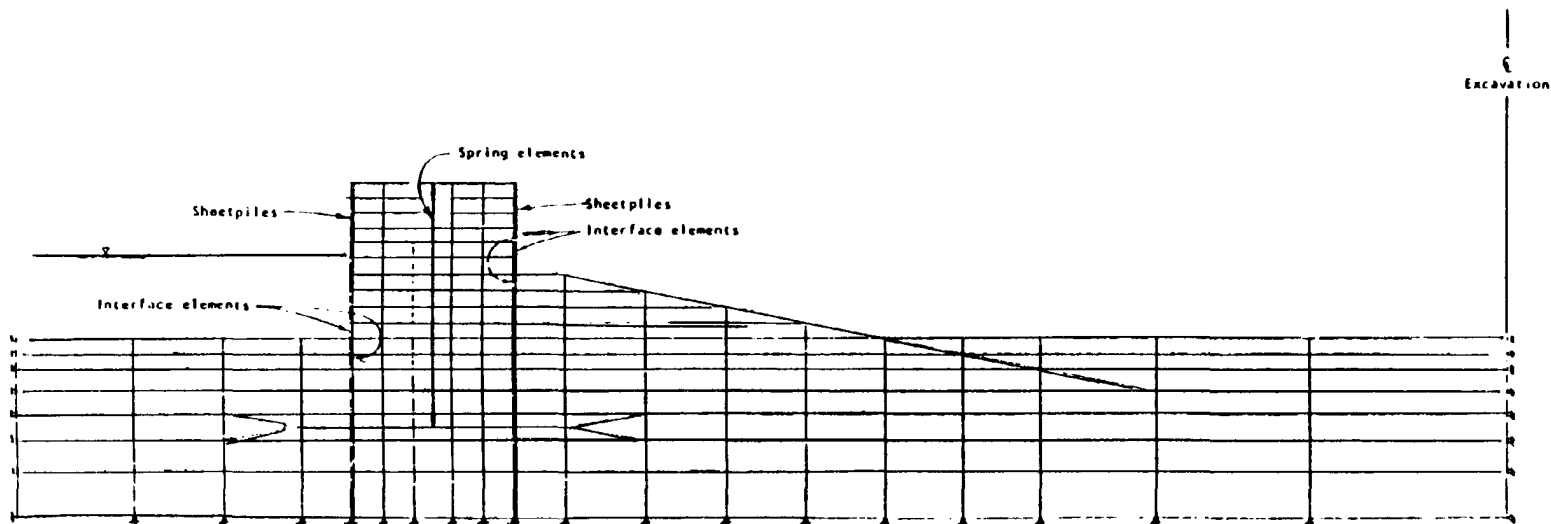
Figure 4-21. Vertical slice analysis, finite element mesh
