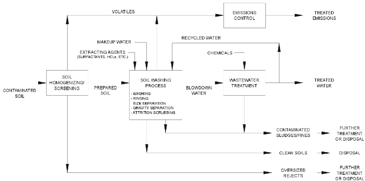
FIGURE 6-1. TYPICAL PROCESS FOR SOIL WASHING
