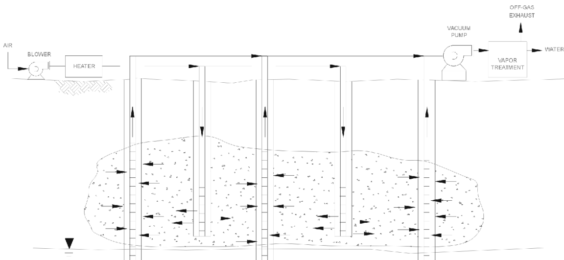
FIGURE 7-1. SVE (IN SITU)/THERMALLY ENHANCED SVE
