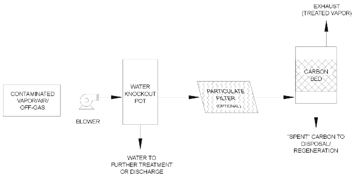
FIGURE 20-1. VAPOR PHASE CARBON ADSORPTION
