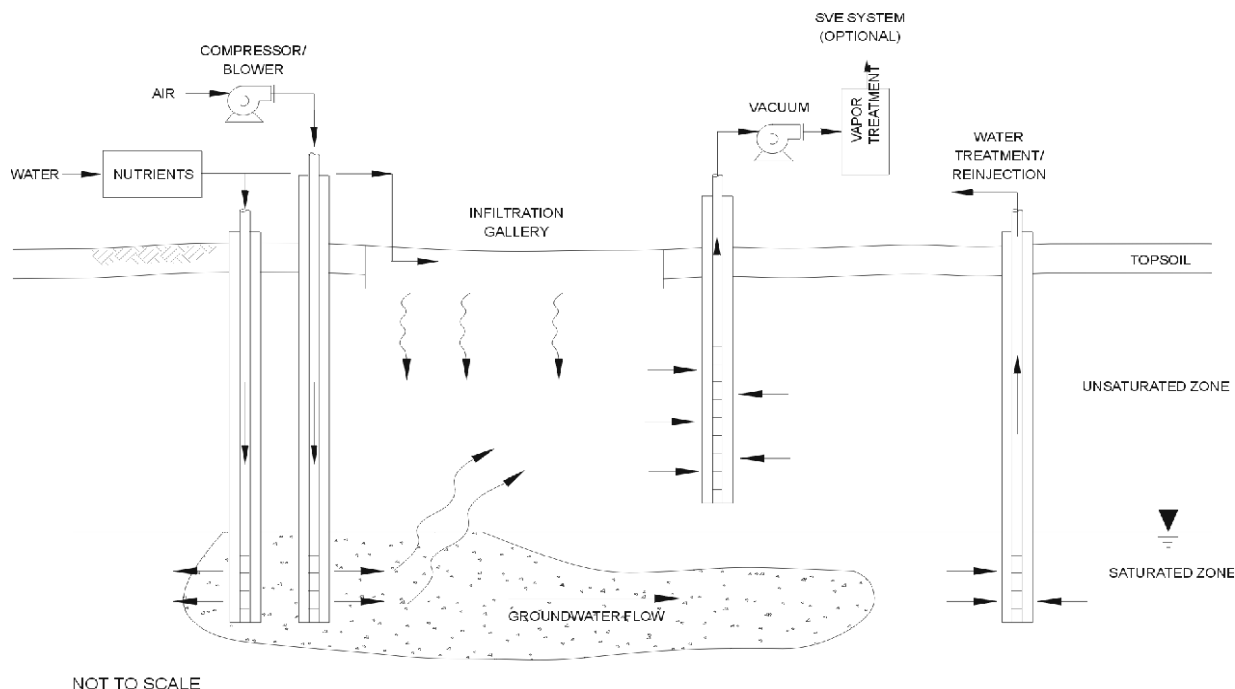
FIGURE 10-1. AIR SPARGING/BIOSPARGING
