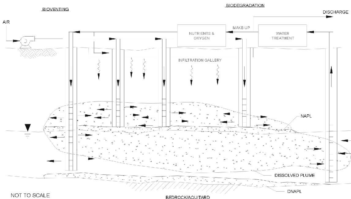
FIGURE 7-2. BIOVENTING/BIODEGRADATION
