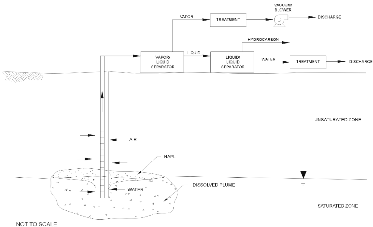
FIGURE 9-1. DUAL-PHASE EXTRACTION/BIOSLURPING
