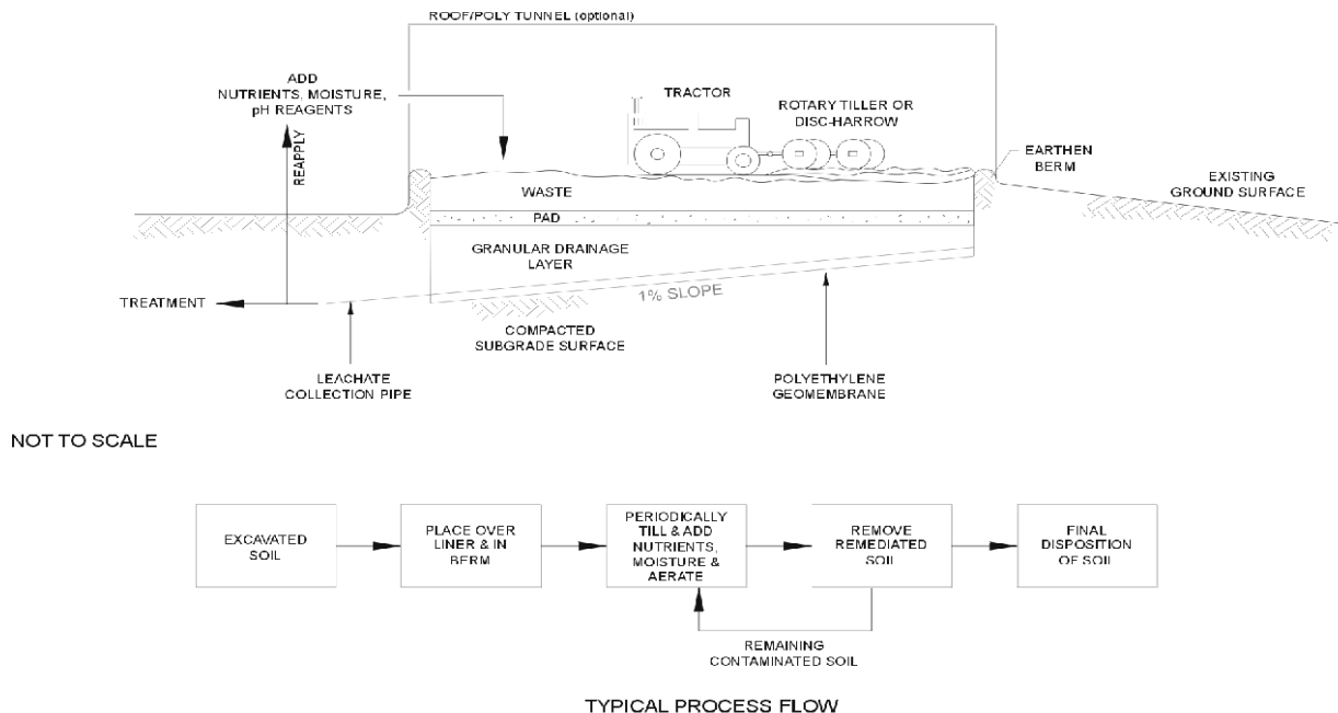
FIGURE 11-1. LANDFARMING
