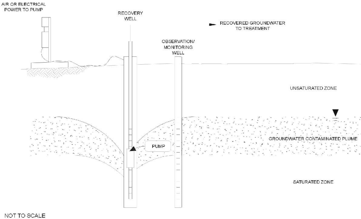
FIGURE 2-1. VERTICAL EXTRACTION WELL
