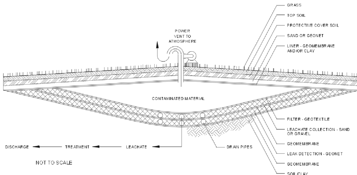
FIGURE 1-1. LANDFILL COVERS/LINERS
